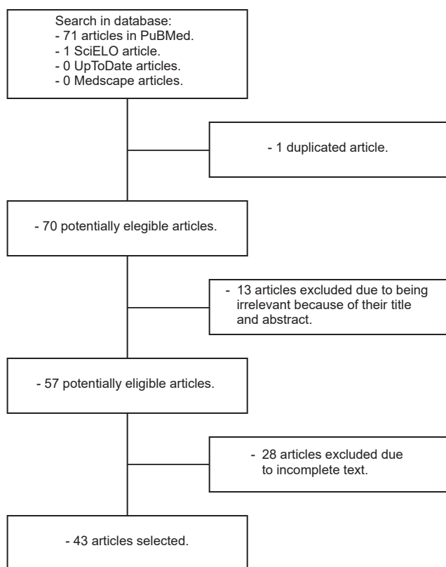
Figure 1. Search algorithm.
