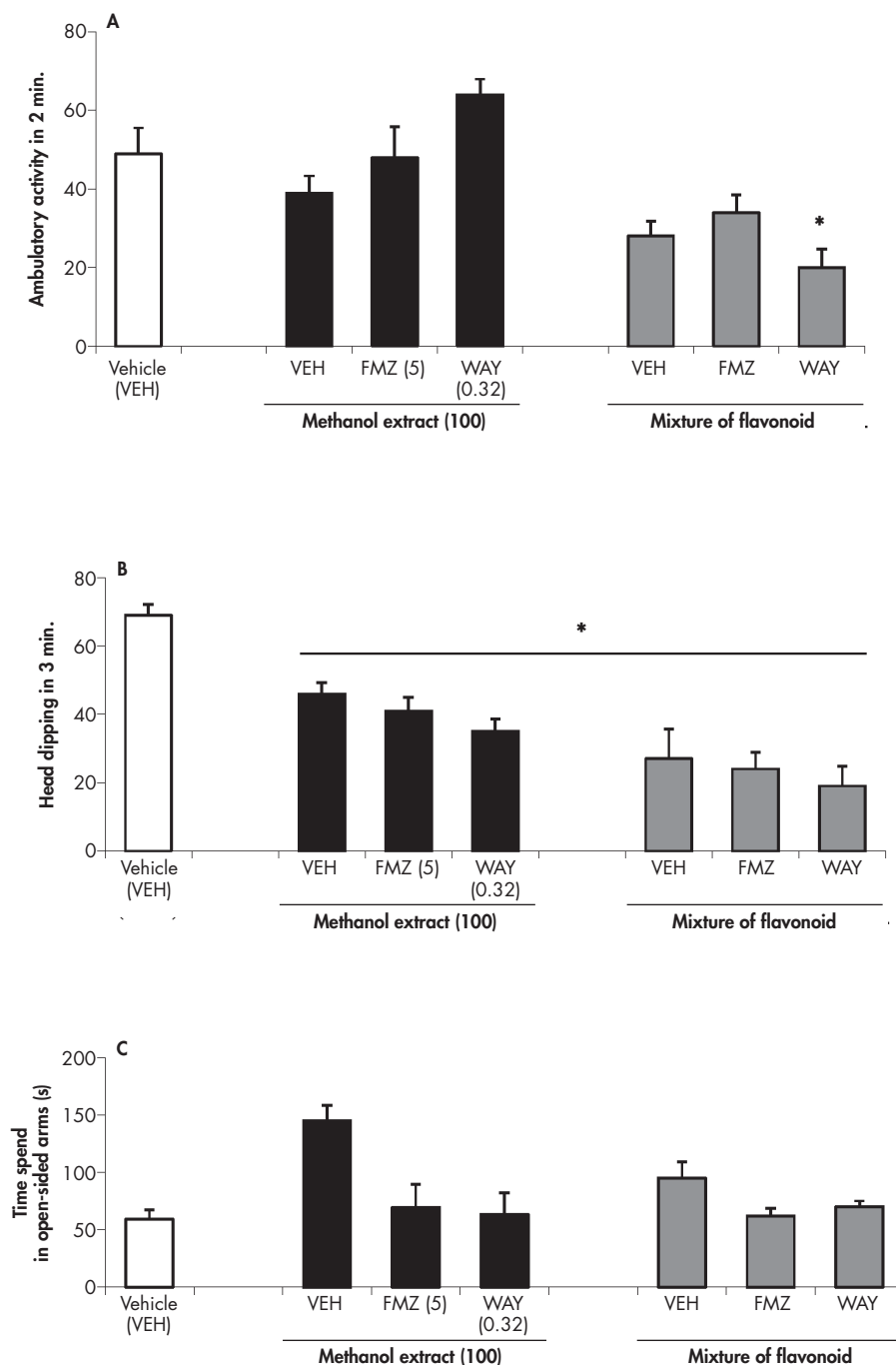
Figure 5. Anxiolytic and sedative-like responses to the methanol crude extract and a mixture of flavonoids composed of quercetin (20 mg/kg), rutin (15.7 mg/kg) and isoquercitrin (2 mg/kg) evaluated in the presence of flumazenil or WAY100635, antagonists of the GABAA/BDZs and 5-HT1A receptors respectively, using the open field (A), hole-board (B) and plus-maze (C) behavior tests. Each bar represents the mean \pm S.E.M. of at least six animals.
