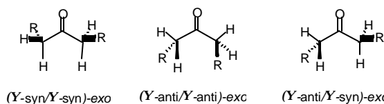
Fig. 1. Preferred conformations for the 1,3-disubstituted acetone fragment.
