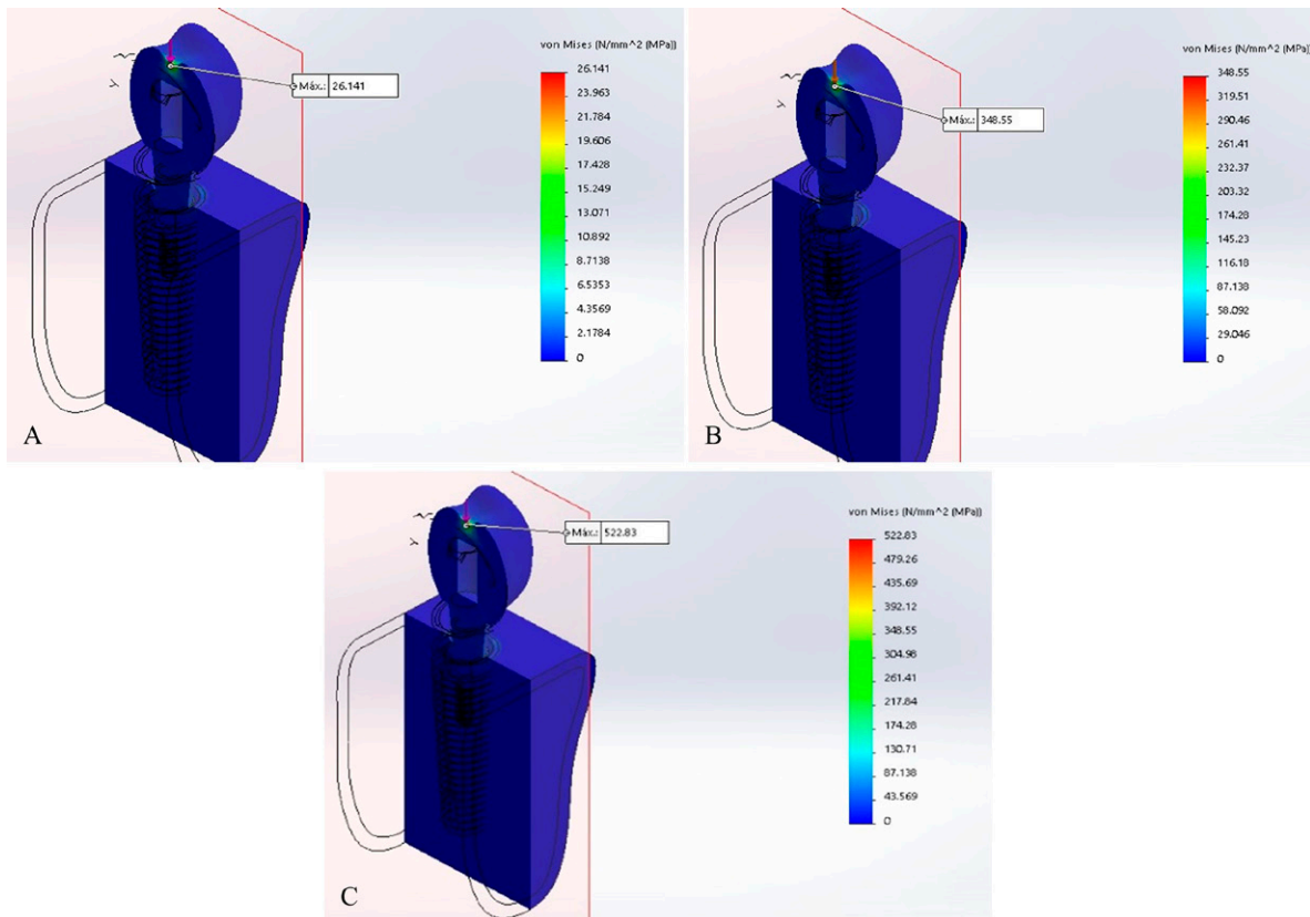
Figure 4. Conventional implant, von Mises with axial force, isometric view in section. A) 7.5 N. B) 100 N. C) 150 N.
