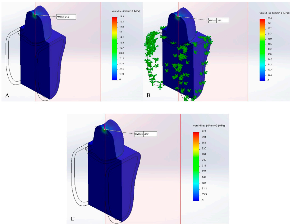
Figure 3. Tooth, von Mises with axial force, isometric view in section. A) 7.5 N. B) 100 N. C) 150 N.
