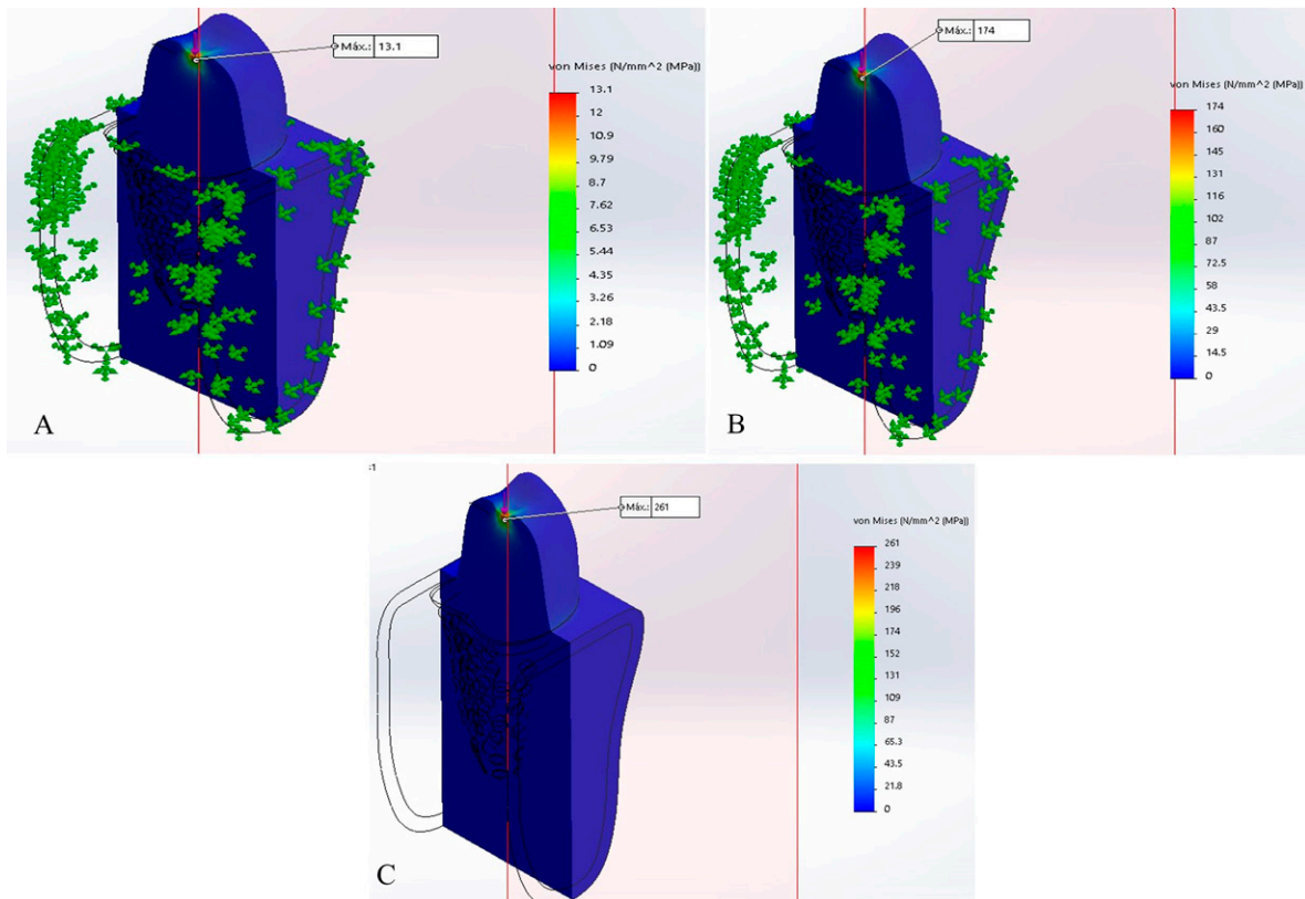
Figure 5. Customized implant, von Mises with axial force, isometric view in section. A) 7.5 N. B) 100 N. C) 150 N.
