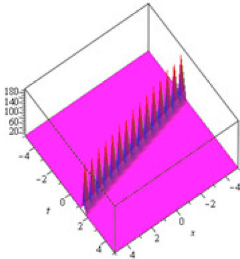
FIGURE 13. The 3D plot of |u_{16}^{\pm}(x, t)| .
