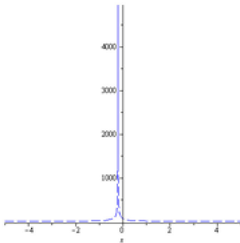
FIGURE 15. The 2D plot of |u_{16}^{\pm}(x, t)| .
