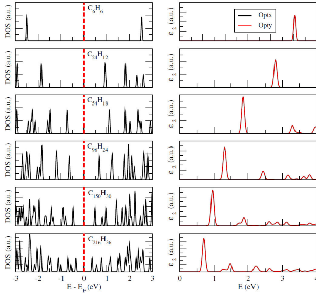
FIGURE 2. Density of states computation, and the imaginary part of the dielectric function, for the hexagonal GQDs depicted in Fig. 1 as the size of the system increases.
