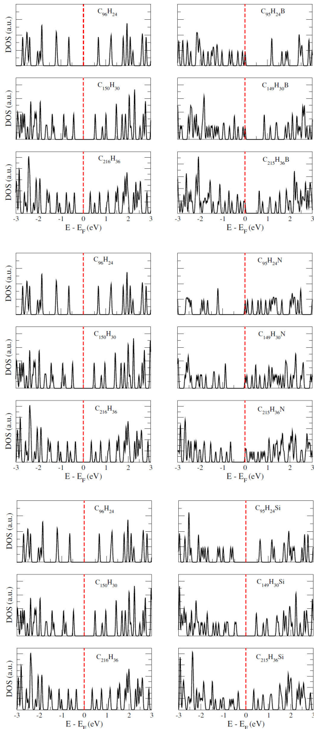
FIGURE 4. Density of states for C_m H_n (left column) and C_{m-1} H_n S_a (right column). Here S_a stands for substitutional atoms of boron (B), nitrogen (N), and silicon (Si). The (m, n) pair values are (96,24), (150,30), (216,36).
