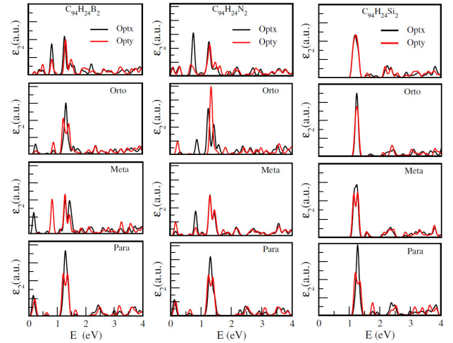
FIGURE 11. Imaginary part of the dielectric function ( \epsilon_2 ), with light polarization in x - and y -directions, with B, N, and Si substitutional atoms at random, ortho -, meta -, and para -director positions.
