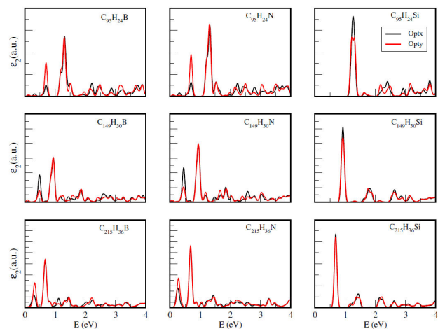
FIGURE 5. Imaginary part of the dielectric function, considering x - and y -direction polarized light, for C_{m-1} H_n S_a . Here, S_a stands for the substitutional atom (B, N, and Si).
