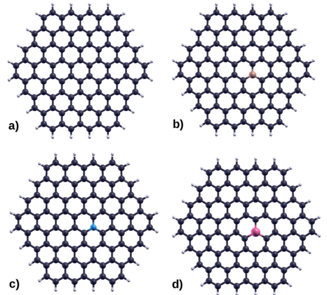
FIGURE 3. Hexagonal C_{96}H_{24} GQD a) without doping, b) considering a B substitutional atom ( C_{95}H_{24}B ), c) a N substitutional atom ( C_{95}H_{24}N ), and d) a Si substitutional atom ( C_{95}H_{24}Si ).
