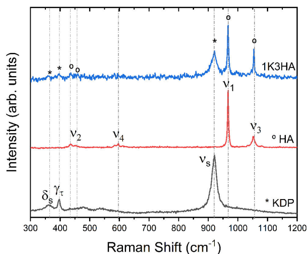
FIGURE 3. Raman spectra comparison of composite with pure KDP, HA and 1K3HA composite.
