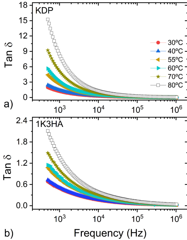
FIGURE 7. Frequency dependence of dielectric loses spectra at a few temperatures for a) KDP and b)13HA composite.
