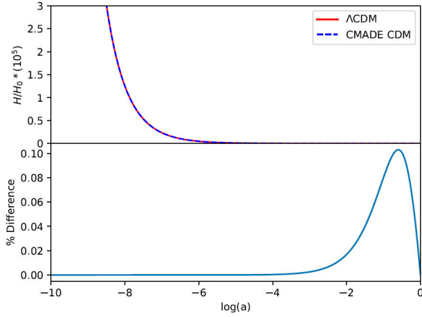
FIGURE 1. In the upper panel we show the evolution of the Hubble parameter using the CMADE (Eq. (4), point line) and the \Lambda CDM model (solid line). We used the Planck values \Omega_{0m} = 0.315 , \Omega_{0r} = 10^{-4} , H_0 = 67.3 km/s/Mpc in both plots and the value \Omega_{0\Lambda} = 0.684 for the \Lambda CDM curve and (7) for the CMADE model. In the lower panel we show the proportional difference between both curves (H_{\text{CMADE}} - H_{\Lambda\text{CDM}})/H_{\Lambda\text{CDM}} .
