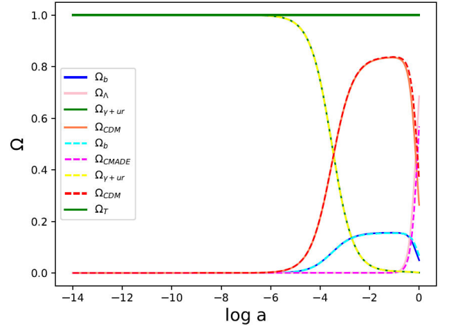
FIGURE 3. Evolution of the \Omega 's using Eqs. (9) and (10) and the corresponding ones using the \Lambda CDM model.
