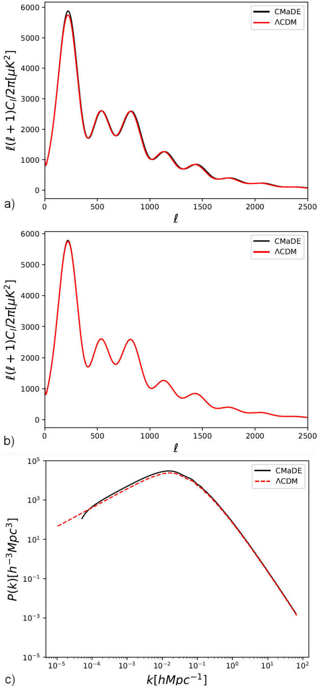
FIGURE 4. Profiles of the CMB for a flat universe (upper panel) and for a closed universe with \Omega_{0k} = -0.003 (middle panel) and MPS (lower panel) observations using an amended version of CLASS code [4]. We compare them with the best fit of the \Lambda CDM model, using data from the Planck satellite. Note that the CMB temperature fluctuations for the flat universe are the same as the \Lambda CDM, the only difference is in the first maximum. For the MPS there are very small discrepancies for the small structure. The CMaDE model settings are \Omega_{0r} = 5.67 \times 10^{-5} , q = 0.694 , H_0 = 72.6 km/s/Mpc and \Omega_{0b} = 0.044 for the flat universe and q = 0.695 , \Omega_{0k} = -0.003 , H_0 = 72.6 km/s/Mpc and \Omega_{0b} = 0.043 for the closed universe. Observe that the value of H_0 is very close to the observed one from the local distance ladder [5].
