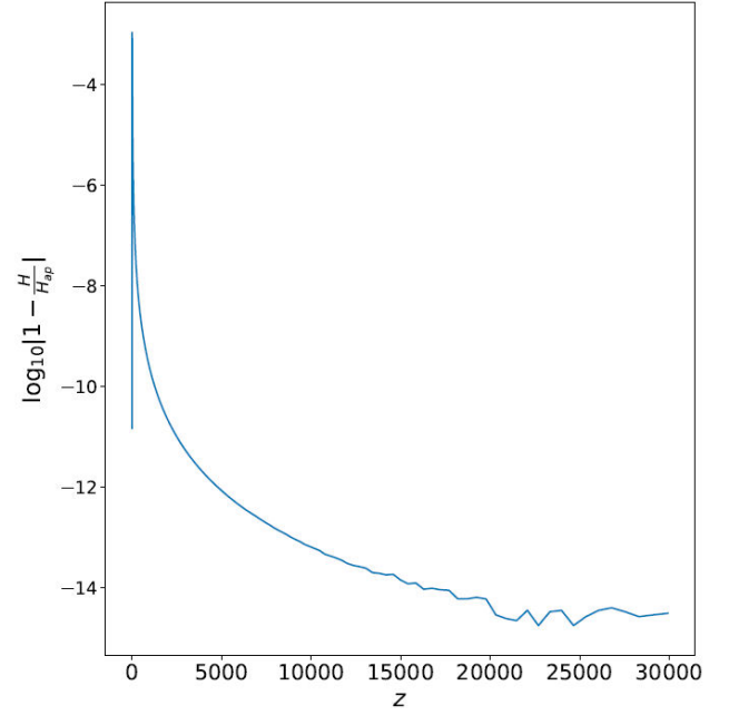
FIGURE 2. Evolution of the 1 - H/H_{app} using the numerical integration of Eq. (4) ( H ) and (10) ( H_{app} ), with q = 0.695 . We plot \log(|1 - H/H_{app}|) , observe that this ratio is always less than 10^{-3} .
