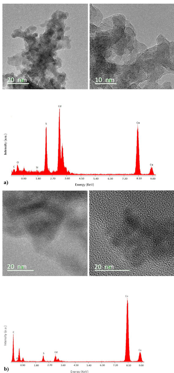
FIGURE 2. TEM images and TEM elemental analysis of a) CdS nanoparticles, b) P3HT/CdS nanocomposite. Right side, bright field TEM images.
