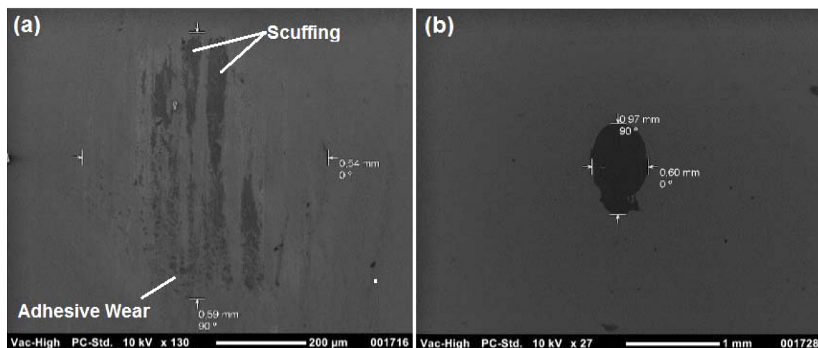
FIGURE 10. SEM micrographs at 50 cycles: (a) the 316 LVM substrate; (b) coated specimen with TiNbCN n = 200 .
