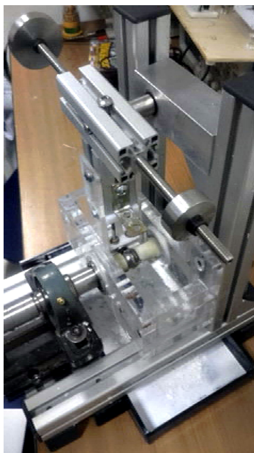
FIGURE 2. Micro-abrasion-corrosion equipment.
