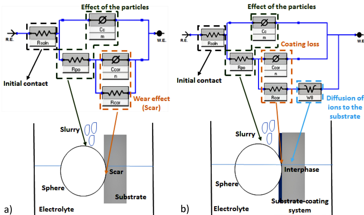
FIGURE 14. Electric circuits of the electrochemical behavior: (a) 316 LVM steel substrate and (b) the substrate coated with TiNbCN n = 200 .
