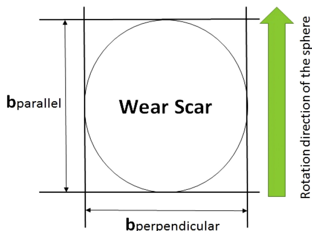
FIGURE 1. Measurement on wear scar.
