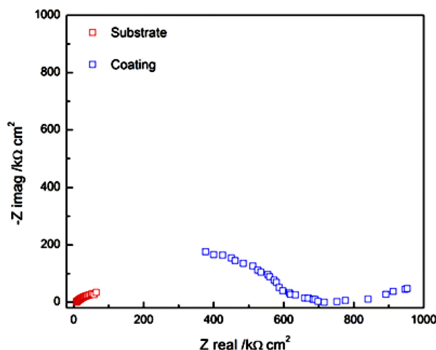
FIGURE 13. Electrochemical impedance spectroscopy (Nyquist diagrams) for the 316 LVM steel substrate and the substrate coated with TiNbCN n = 200 .
