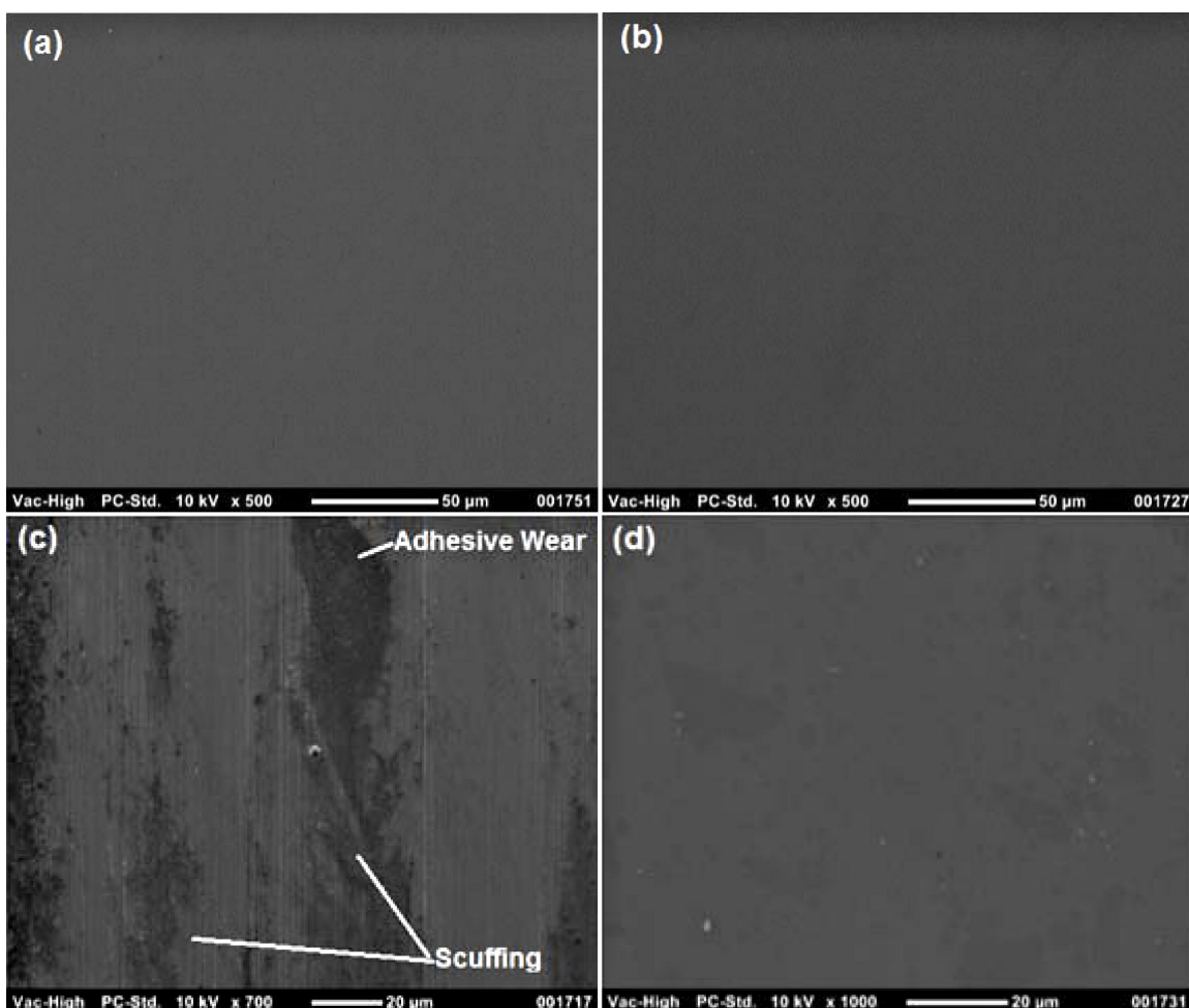
FIGURE 8. Surface of the specimens without micro-mechanism of: (a) 316 LVM steel substrate, (b) 316 LVM steel substrate coated with TiNbCN n = 200 . Wear surface at 50 cycles: (c) 316 LVM steel substrate, (d) 316 LVM steel substrate coated with TiNbCN n = 200 .
