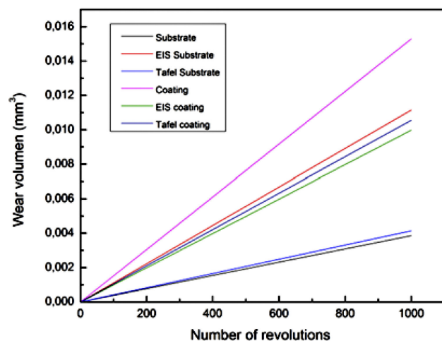
FIGURE 11. Wear volume vs number of revolution: for 316 LVM substrate and 316 LVM substrate coated with TiNbCN n = 200 , subjected to micro-abrasion-corrosion.
