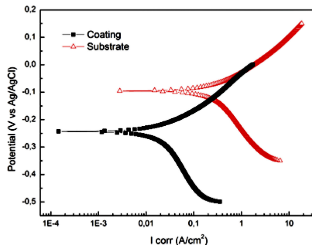
FIGURE 12. Tafel polarization curves, for the 316 LVM substrate and coated specimen with TiNbCN n = 200 .
