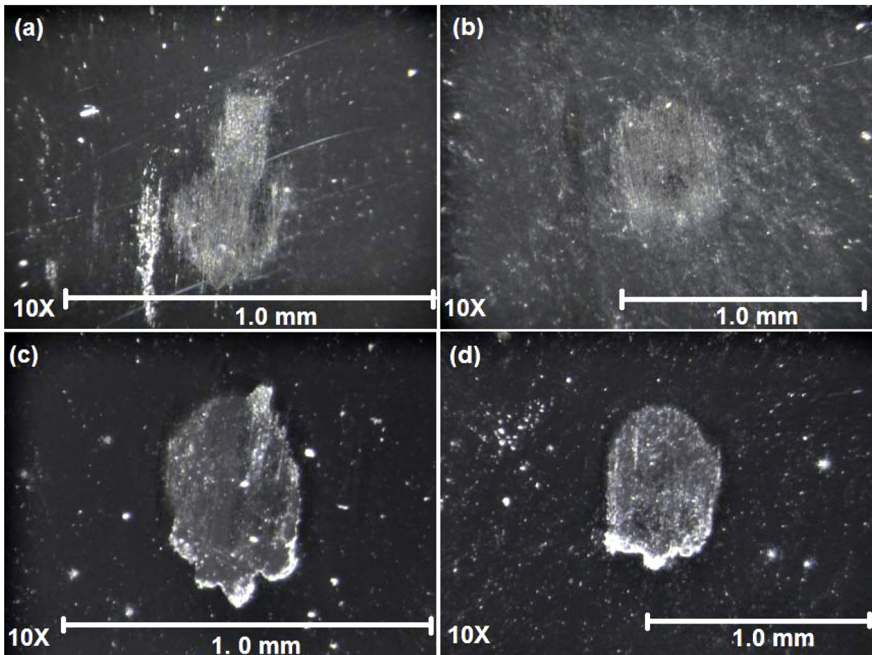
FIGURE 7. Wear scars of the micro-abrasion-corrosion tests by stereographic microscopy: (a) 316 LVM steel substrate subjected to EIS, (b) 316 LVM steel substrate subjected to Tafel, (c) 316 LVM steel substrate coated with TiNbCN n = 200 subjected to EIS, and (d) 316 LVM steel substrate coated with TiNbCN n = 200 subjected to Tafel.
