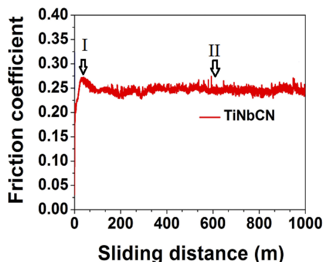
FIGURE 5. Tribological results of TiNbCN coating (friction coefficient as a function of sliding distance).
