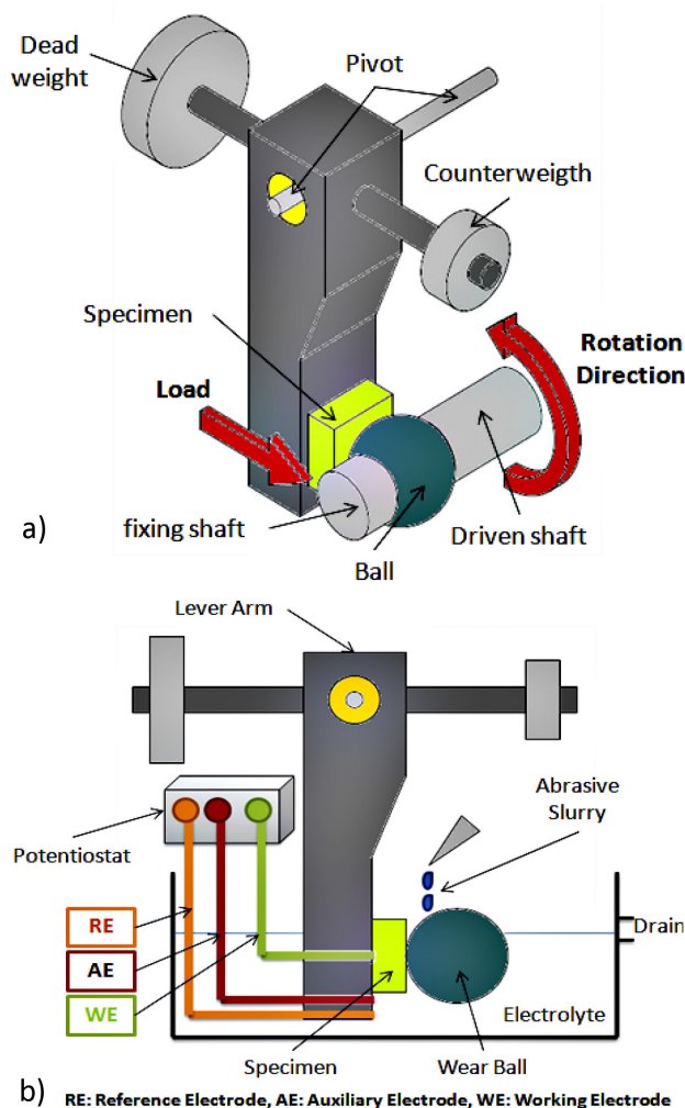
FIGURE 3. Schematics representation of the tests (a) micro-abrasion; (b) micro-abrasion-corrosion.
