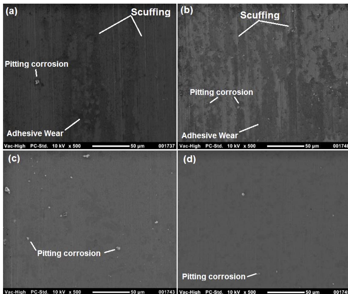
FIGURE 9. Tribo-chemical wear scars by SEM where is observed the adhesive wear, micro-abrasion and pitting corrosion: (a) 316 LVM steel substrate subjected to EIS, (b) 316 LVM steel substrate subjected to Tafel, (c) 316 LVM steel substrate coated with TiNbCN n = 200 subjected to EIS, and (d) 316 LVM steel substrate coated with TiNbCN n = 200 subjected to Tafel.
