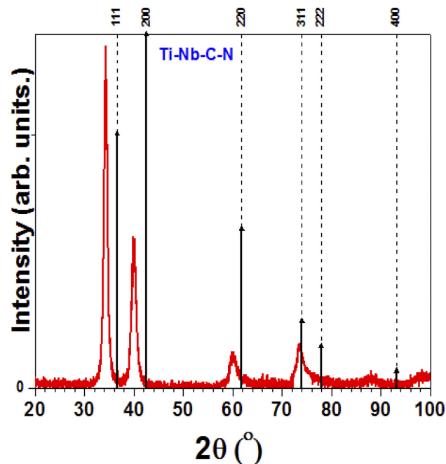
FIGURE 4. XRD pattern for: Ti-Nb-C-N coatings grown with an r.f. negative bias voltages of -20 V. Dash lines indicate the position of the peaks obtained from JCPDF files.
