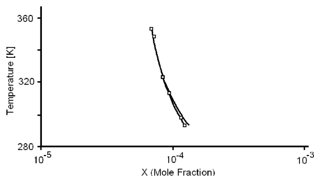
FIGURE 5. The horizontal coordinate corresponds to the mole fraction of asphaltene in toluene. All cmc square points of Rogacheva et al. [6] were reproduced using \gamma = 10.4038 , \beta C = 293/\gamma T and K = 500 ). A small improvement of \beta C or K will provide just one calculated curve.
