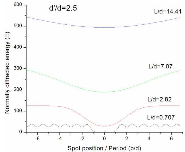
FIGURE 12. Normally diffracted energy as a function of the spot position ( b/d ) for a normally incident Gaussian beam on an aperiodic ruling with d=1.0 and d'=2.5 , with wavelength \lambda = 0.01 .
