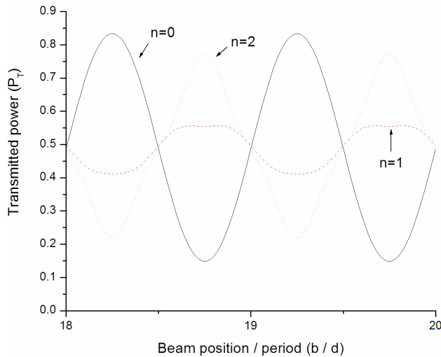
FIGURE 2. Transmitted power as a function of the beam position for Hermite-Gaussian beams of order n=0 (solid line), 1 (dash line), and 2 (dot line), with width L/d = 0.5 , and \lambda/d = 0.03 .
