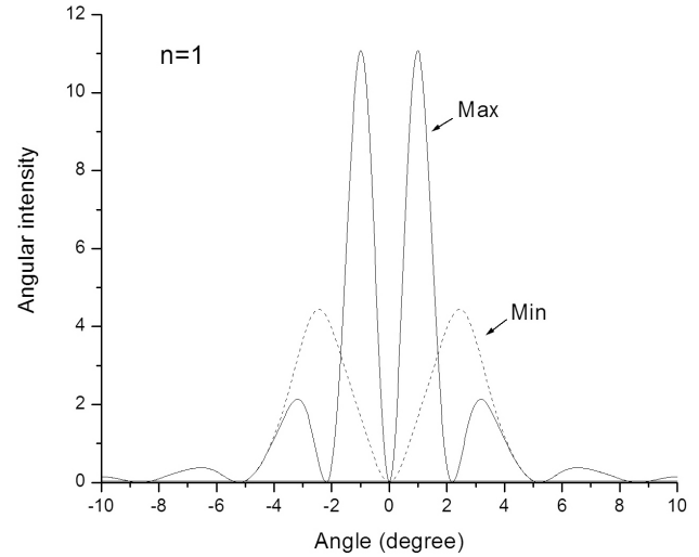
FIGURE 6. Same as Fig. 5 but for n = 1 .
