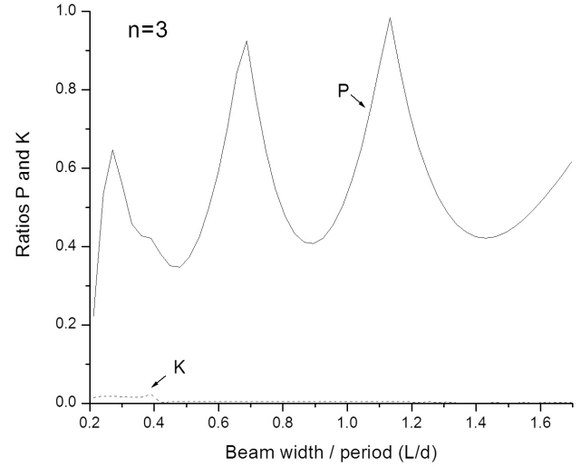
FIGURE 11. Same as Fig. 8 but for n = 3 .
