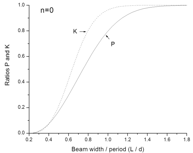
FIGURE 8. Intensity ratio K = E_{\min}/E_{\max} (dashed curve) and P = P_{\min}/P_{\max} (solid curve) for a normally incident Gaussian beam as functions of the normalized beam width L/d , for a Ronchi ruling with period d = 1.0 .
