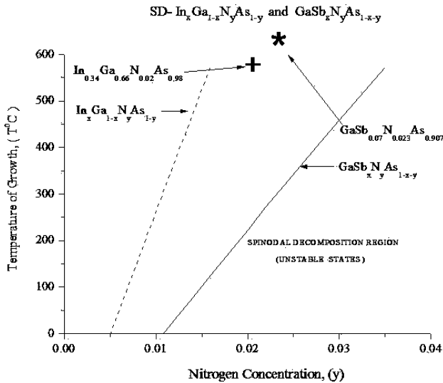
FIGURE 1. The spinodal decomposition ranges of the GaAs-enriched \text{GaSb}_x\text{N}_y\text{As}_{1-x-y} and \text{In}_x\text{Ga}_{1-x}\text{N}_y\text{As}_{1-y} alloys. \text{In}_{0.34}\text{Ga}_{0.66}\text{N}_{0.02}\text{As}_{0.98} and \text{GaSb}_{0.07}\text{N}_{0.023}\text{As}_{0.907} are the experimental values.
