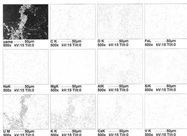
FIGURE 7. Micrograph of the elemental distribution (mapping) of uranium and potassium concentration in the same zone, obtained by SEM, coupled with a system of X-ray dispersive energy. The mineral is uranophane.
