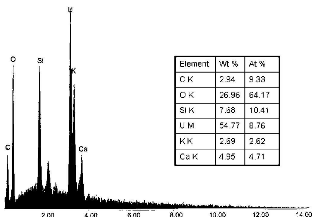
FIGURE 5. SEM microprobe spectrum of a sample collected in the San Marcos zone, where it is observed the presence of uranium and potassium. Ordinate axis is in arbitrary units and abscissas are X-ray energies in keV.
