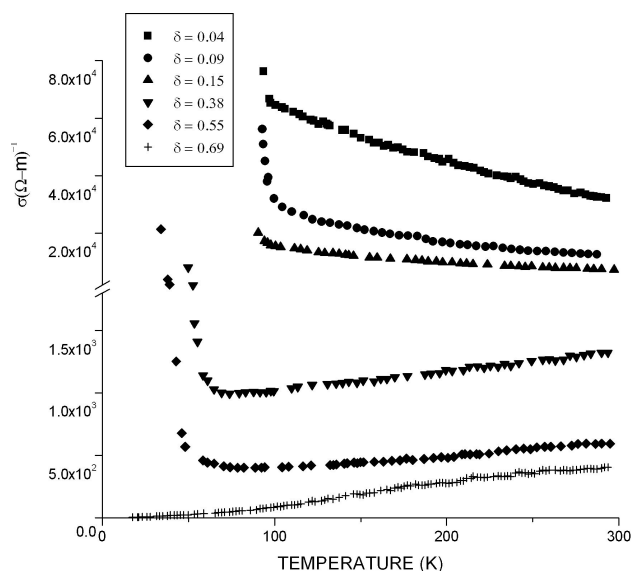
FIGURE 1. Electric conductivity versus temperature in samples of \text{EuBa}_2\text{Cu}_3\text{O}_{7-\delta} for several oxygen concentrations, 7 - \delta .
