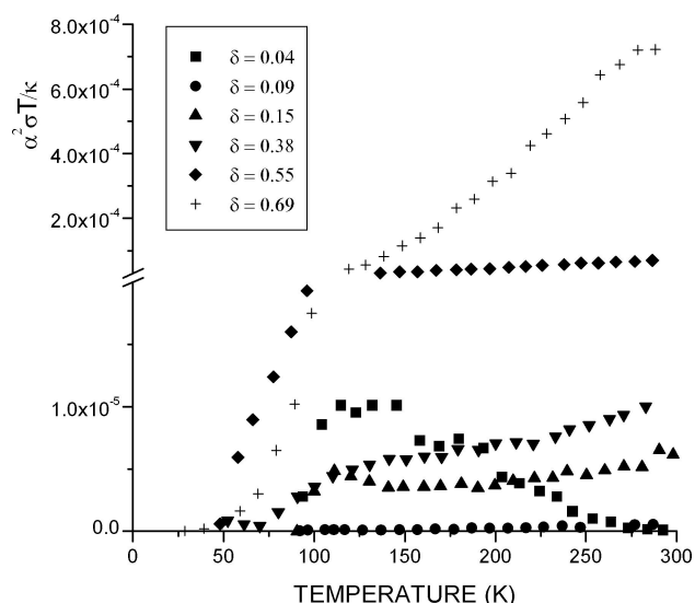
FIGURE 2. Figure of merit of \text{EuBa}_2\text{Cu}_3\text{O}_{7-\delta} for several oxygen concentrations, 7 - \delta , at low temperature.
