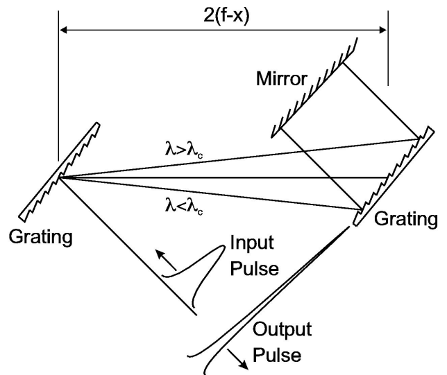
FIGURE 6. The compressor has two diffraction gratings to revert the chirp introduced in the stretcher stage, and compensate for dispersion introduced by the components of the amplifier system.
