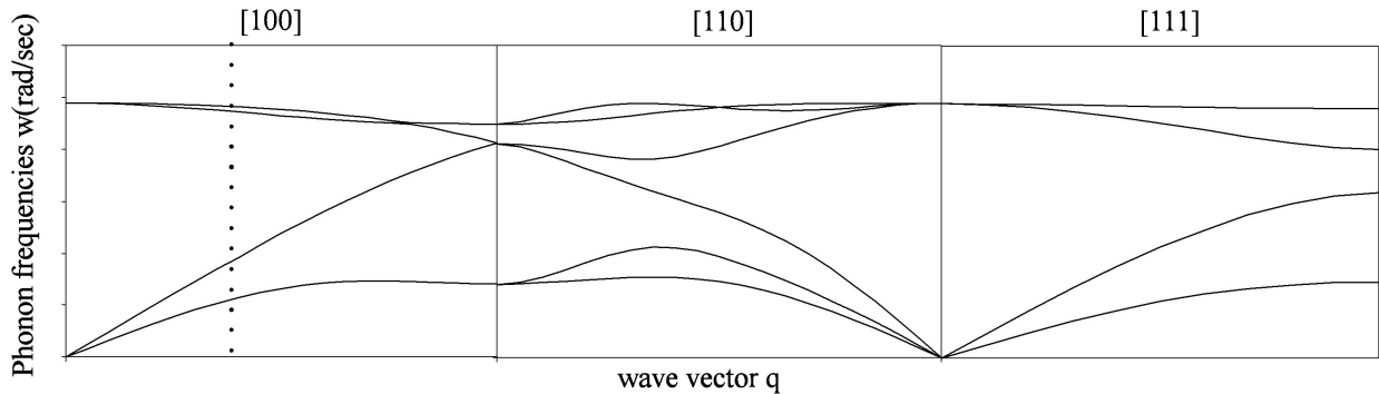
FIGURE 1. Phonon dispersion curves for silicon using Wanser model, the dotted lines indicate possible channels of decay.
