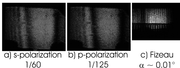
FIGURE 11. Experimental monochromatic multiple beam interference patterns for low value of \theta . s - polarization (thin line) and p - polarization (thick line), both taken with f/3.6 aperture at \lambda = 632.8 nm. Exposure times 1/60 ( s ) and 1/125 ( p ). c) two-beam Fizeau interference pattern (dashed line) at \lambda = 543.5 nm.
