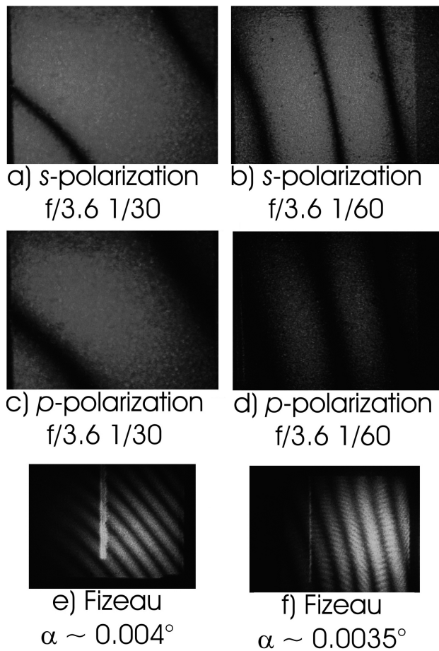
FIGURE 13. Experimental monochromatic interference patterns for larger values of \theta : (a) and (b) under s -polarization, while (c) and (d) under p -polarization. a), c) and e) the same value of \theta and \alpha . b) d) and f) with the same value of \theta and \alpha . Apertures and exposure times as indicated.
