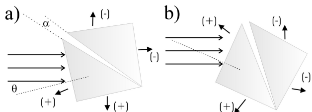
FIGURE 2. An air wedge formed between two prisms. A light beam is incident at angle \theta as shown in the two variants. According to experimental observations, the symbols (+) and (-) denote observed interference patterns of opposite contrasts.
