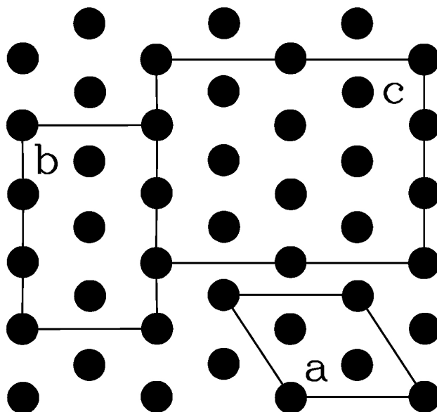
FIGURE 1. Surface cells used in the calculations: (a) (\sqrt{3} \times \sqrt{3}) R30; (b) (3 \times \sqrt{3}) ; (c) (3 \times 2\sqrt{3}) also referred as the c(4 \times 2) superlattice of the (\sqrt{3} \times \sqrt{3}) R30 lattice.
