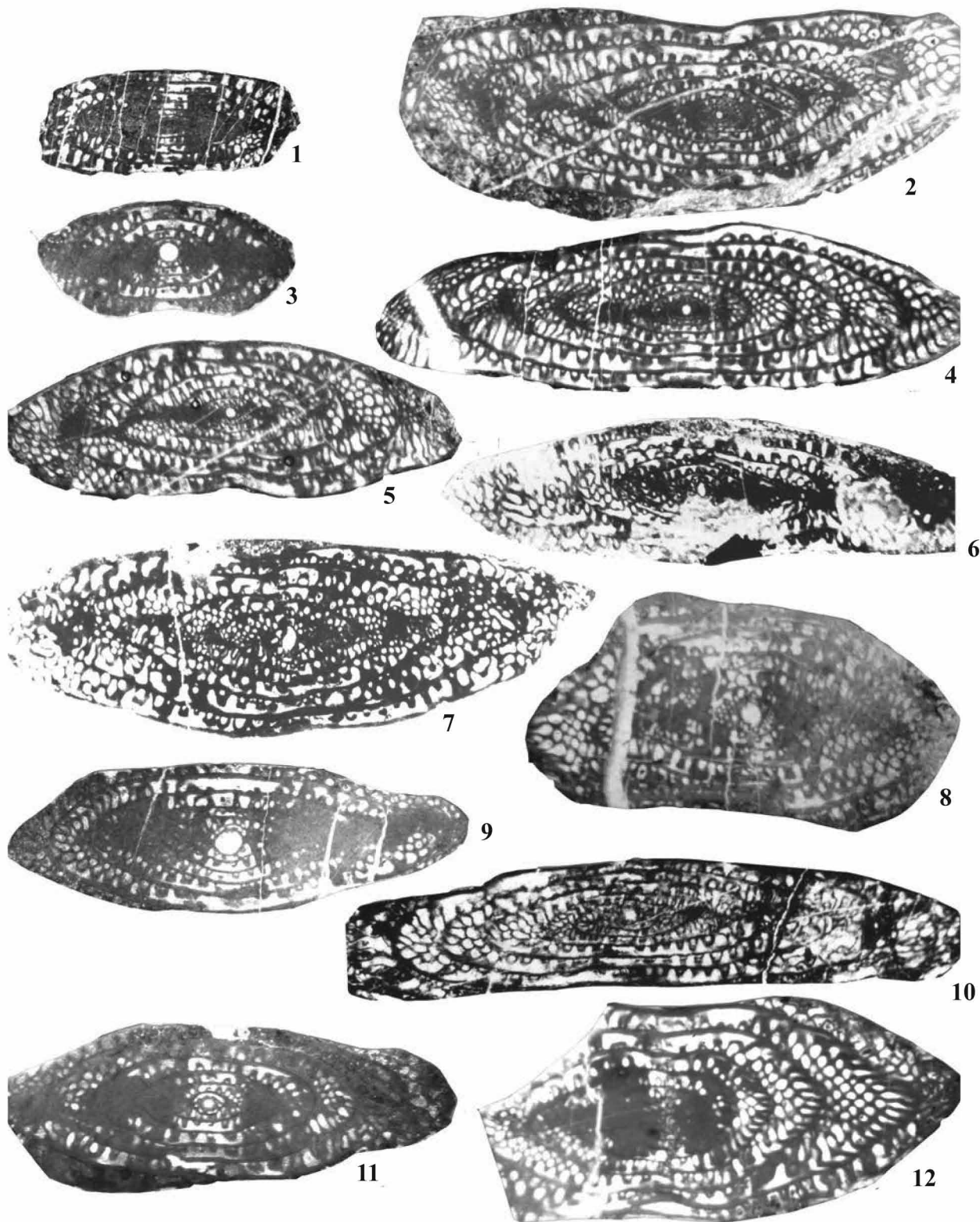
Figure 5. 1-12: Fusulinids from Permian limestones in the Laurentian carbonate shelf (all figures \times 10 ). Permian Shelf Fusulinids: 1 - Pseudochusenella hazzardi , S-2103, slide 390f; 2 - Parafusulina multisepta , S-1628, slide 391f; 3 - Skinnerella cf. S. gruperensis , S-1989, slide 392f; 4 - Parafusulina cf. P. apiculata , S-1628, slide 393f; 5 - Parafusulina apiculata ?, S-1628, slide 394f; 6 - Parafusulina aff. P. allisonensis , S-1879, slide 395f; 7 - Skinnerella sp. A (of Pérez-Ramos, 1992), S-1879, slide 396f; 8 - Skinnerella gruperensis , S-1935, slide 397f; 9 - Skinnerella aff. S. figueroai , S-1989, slide 398f; 10 - Parafusulina leonardensis , S-1806, slide 399f; 11 - Skinnerella cf. S. australis , S-1989, slide 400f; 12 - Parafusulina multisepta , S-1935, slide 401f.
