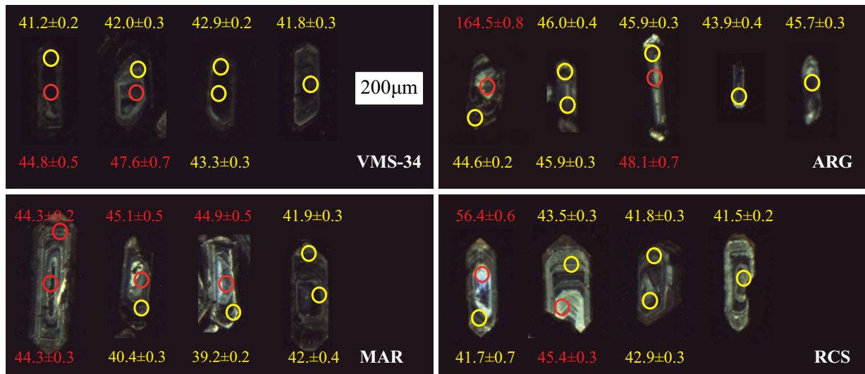
Figure 4. Cathodoluminescence images of the zircon dated. The white bar corresponds to a 200 \mu m scale. The spot is 34 \mu m in diameter. The reported ages are ^{206}Pb/^{238}U ages. Ages in yellow are used to calculate the sample age. The ages in red are from inherited zircon cores, not used in the calculated age.
