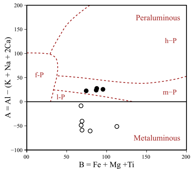
Figure 7. A-B plot (modified by Villaseca et al. , 1998), with A=[Al-(K+Na+2Ca)] and B=Fe+Mg+Ti (gram-atoms \times 10^3 of each element in 100 g of material). Note that all the Sierra de Catorce samples (black dots) are moderately peraluminous, while the Sierra El Fraile samples (open dots) from Pinto-Linares et al. (2008) are metaluminous. f-P: highly felsic peraluminous; l-P: low peraluminous; m-P: moderately peraluminous; h-P: highly peraluminous.
