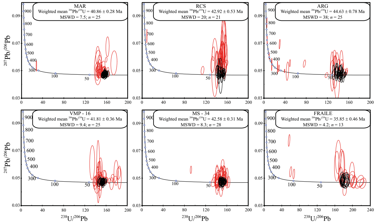
Figure 3. Concordia diagrams of the six samples dated by LA-ICPMS. Concordia, ages and errors are calculated using Isoplot 3.71 (Ludwig, 2008). Ellipses are 1-sigma errors. The ellipses in black correspond to the analysis used for the weighted mean age determination.
