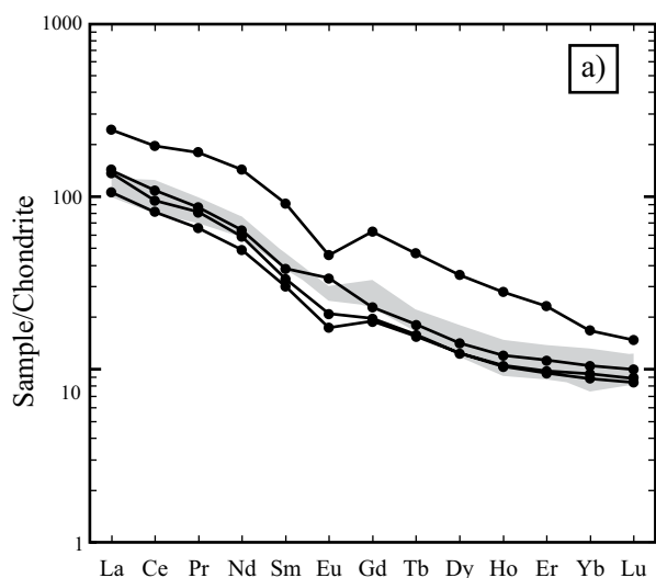
Figure 9. a) Chondrite-normalized (Sun and McDonough, 1989) REE patterns and (b) multi-element plots for Real de Catorce granitoids normalized to primitive mantle (Sun and McDonough, 1989). In both diagrams the shaded area represents the composition of the Sierra del Fraile granitoids (Pinto-Linares et al. , 2008).
