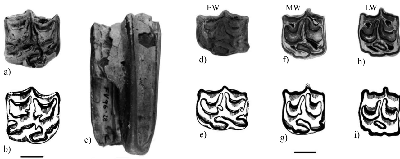
Figure 2. Upper dentition of Pliohippus sp. from the Middle Miocene of Oaxaca, southeastern Mexico. a: occlusal view of IGM 6739 (RP4); b: schematic occlusal representation of same; c: lateral view of same; d, f and h: occlusal views of cross-sectioned specimen IGM 6721 (LP3) at early wear (EW), moderate wear (MW) and late wear (LW); e, g and i: schematic occlusal representations of same. Scale bar equal 1 cm.
