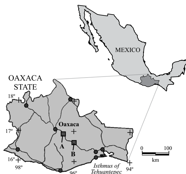
Figure 1. Index map showing the location of the study areas in Oaxaca, southeastern Mexico. A, Matatlán Area, Valles Centrales Region. B, Nejapa de Madero Area, Subisthmian region.
