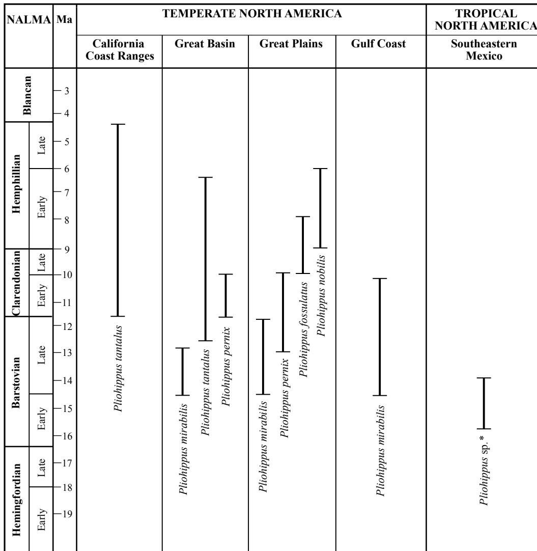
Figure 4. Geographic distribution and geochronological range of known species of Pliohippus from the late Neogene of temperate North America and tropical North America. NALMA refers to North America Land Mammal Ages and modified from Tedford et al. (2004). Geochronological range of the considered species from MacFadden (1998). * present study.
