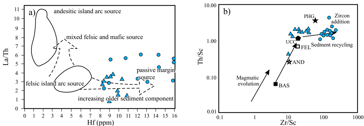
Figure 8. a) Source rock Hf–La/Th— discrimination diagram for the discussion of the clastic sediments and their compositions (Floyd and Leveridge, 1987) for Upper Devonian sandstones from Ilanqareh Formation at Ilanlu and Ilanqareh sections. Symbols as Figure 5. b) Plot of Th/Sc versus Zr/Sc of Upper Devonian sandstones from Ilanqareh Formation (modified after McLennan et al. , 1993). The Upper Devonian sandstones are enriched in zircon, due to sedimentary sorting and recycling. Legend: PHG= Phanerozoic granite; FEL= felsic volcanic rock; AND= andesite; BAS= basalt (igneous rock averages from Condie, 1993); UCC= Upper Continental Crust (composition after Taylor and McLennan, 1985). The lower and intermediate arrows (compositional trend) define the trend expected in first-cycle sediments due to magmatic evolution from mafic to felsic; upper arrow shows the trend produced by the addition of zircon during sedimentary sorting and recycling. Symbols as Figure 5.
