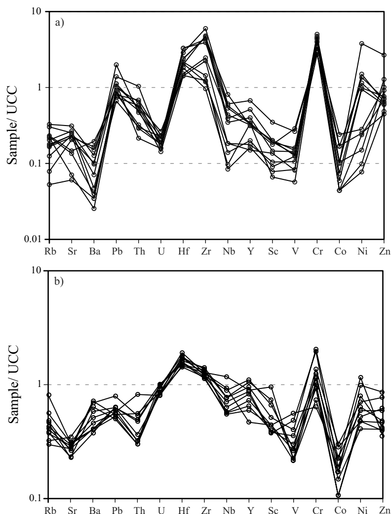
Figure 6. Multi-element normalized diagrams for sandstones of Ilanqareh Formation normalized against average upper continental crust (Taylor and McLennan, 1985).
