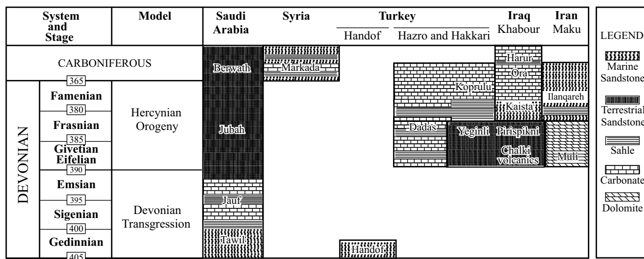
Figure 2. Correlation chart of the Devonian rock units in NW Iran, Saudi Arabia, Turkey, Iraq and Syria, compiled from Hussein (1991).
