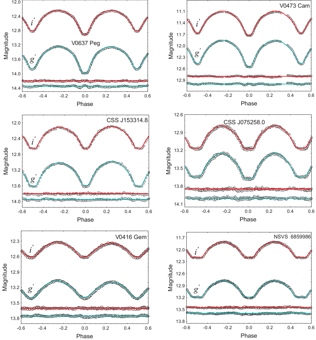
Fig. 1. The folded light curves of the observation targets with their fits and residuals (shifted vertically by different amounts to save space).
