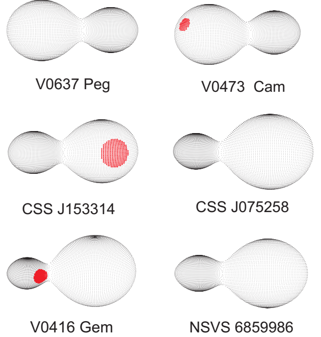
Fig. 2. 3D configurations of the targets.
