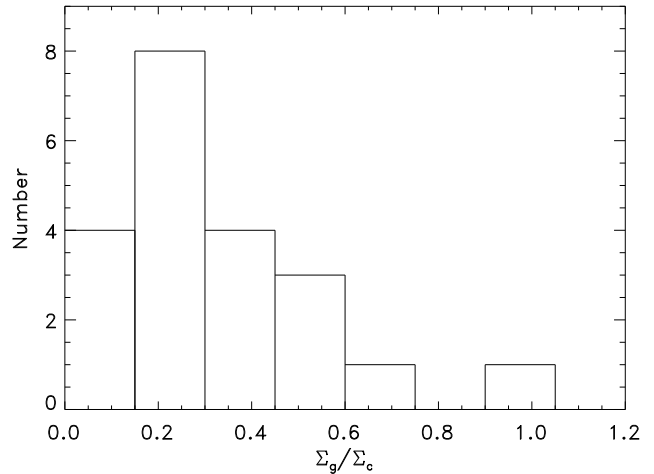
Fig. 3. Histogram of the values of \Sigma_g/\Sigma_c at the radius where \text{SFR} = 10^{-4} M_{\odot} \text{yr}^{-1} \text{kpc}^{-2} in the 21 galaxies with all the required data presented in Leroy et al. (2008).
