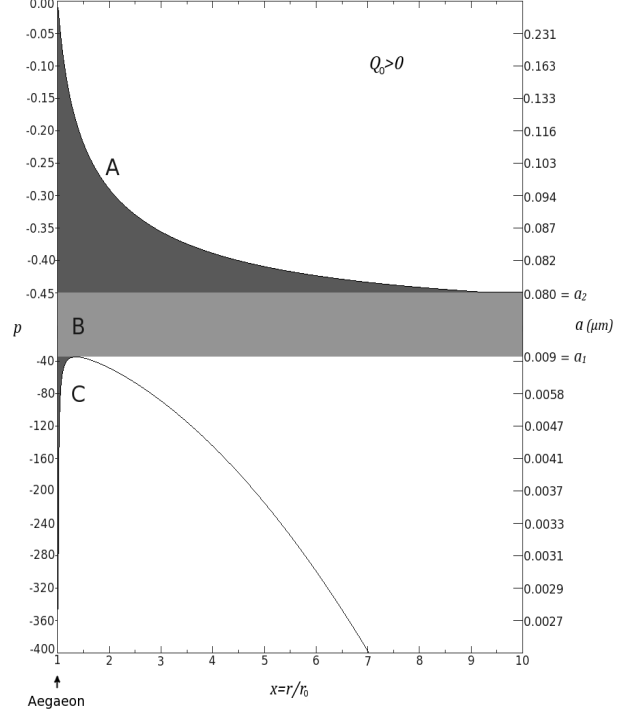
Fig. 3. The confinement and capture regimes for positively charged particles ( Q_0 > 0 and p < 0 ) ejected from Aegaeon surface. A and C represent, the dust confinement regimes and B contains escaping dust grains.
