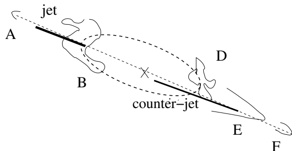
Fig. 3. Schematic diagram of the observed structures.
