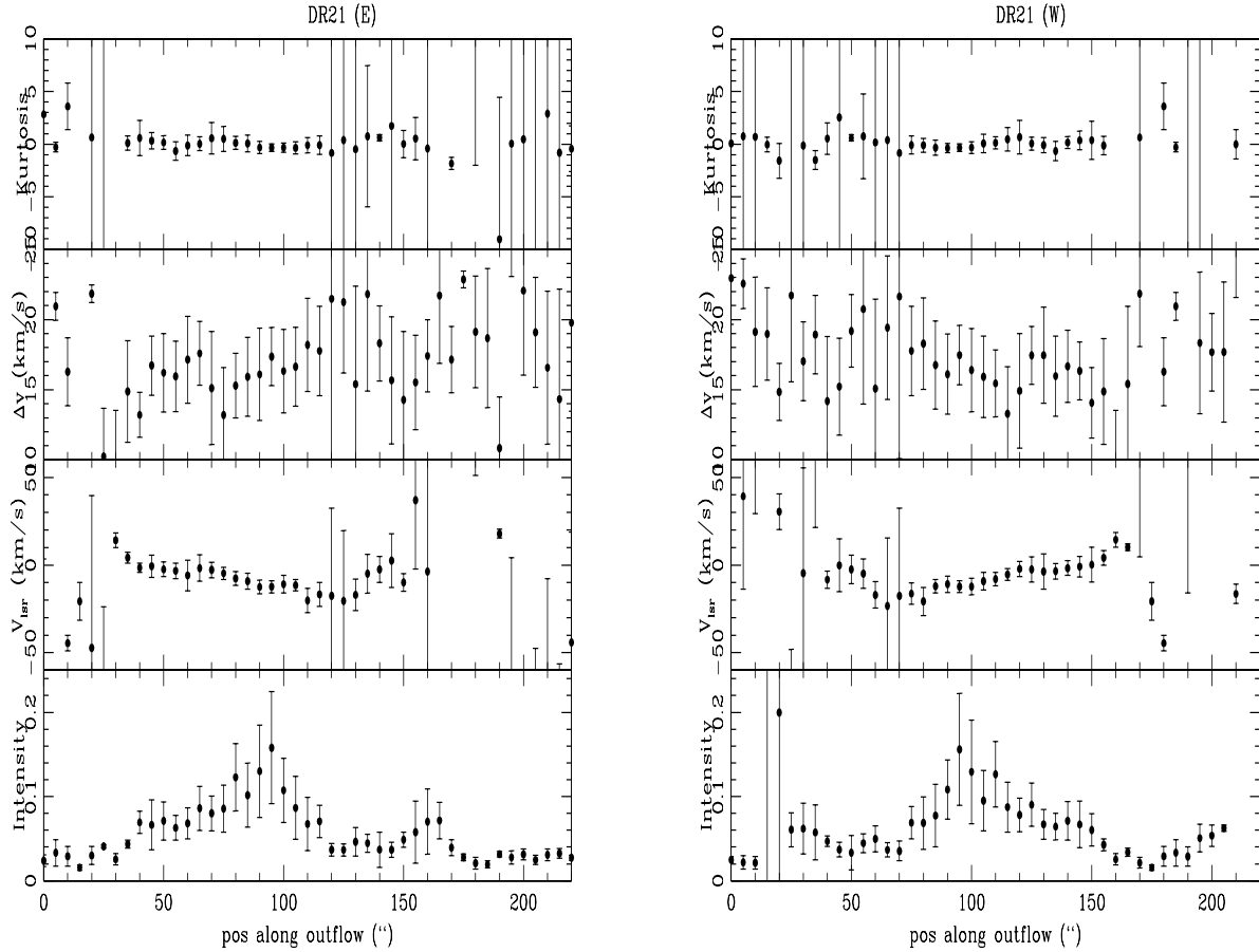
Fig. 7. Velocity moments along the outflow DR 21 (E), from bottom to top: intensity, centroid velocity, velocity dispersion and kurtosis for DR 21 (E) (left) and DR 21 (W) (right).
