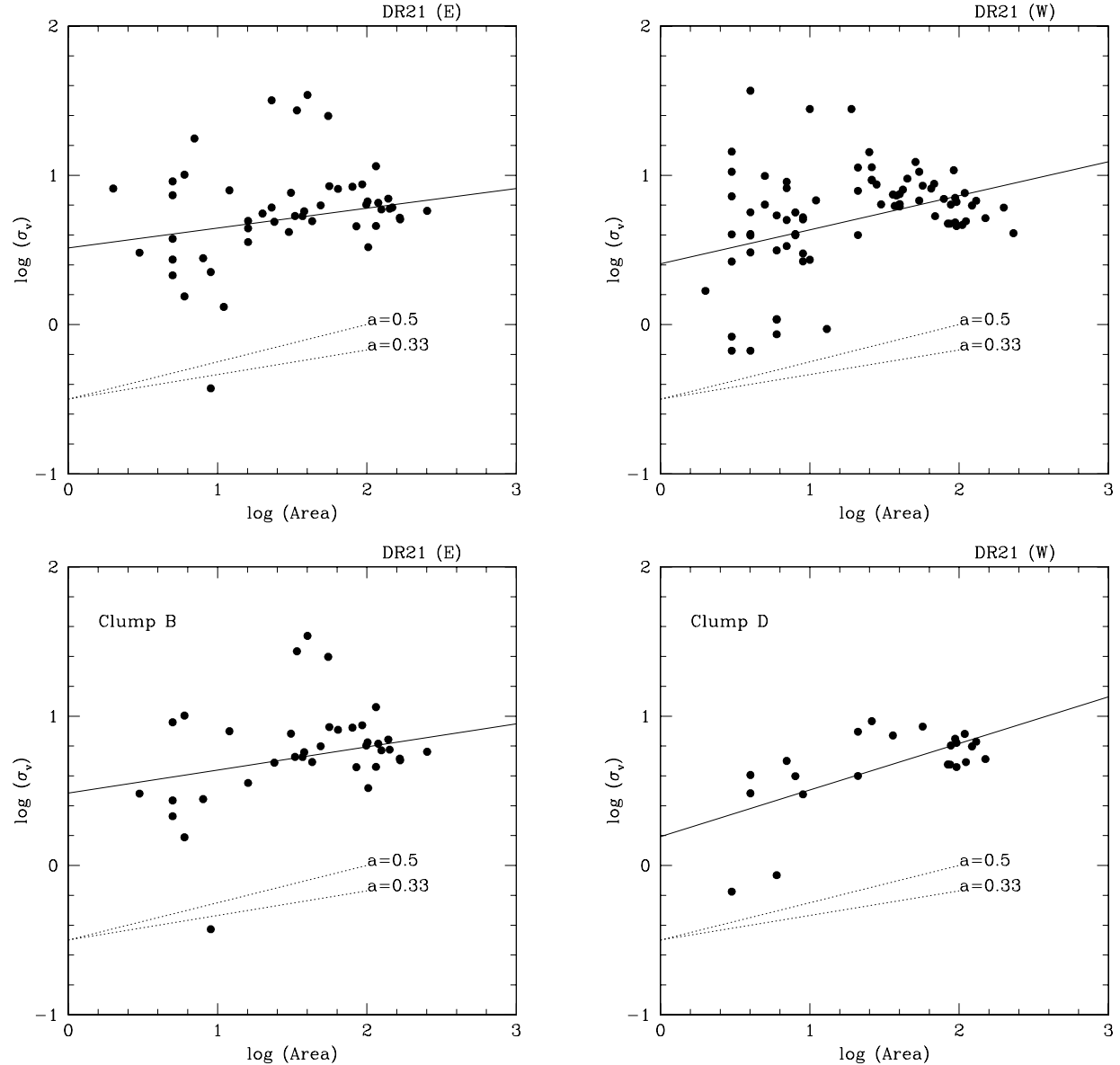
Fig. 9. Clump velocity dispersion \sigma_v vs. clump area for DR 21 (E) (left) and DR 21 (W) (right). Clumps B in DR 21 (E) (left) and D in DR 21 (W) (right) are shown in the bottom panels. In all the panels a solid line represents a linear least-square fit to the data. The two line segments below are the representative power-law indices corresponding to slope a values of 0.33 for a Kolmogorov turbulence and 0.5 for a more virialized gas.
