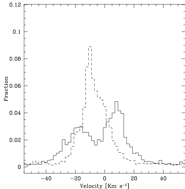
Fig. 4. Fraction of pixels with a given value of the centroid radial velocity (LSR) for DR 21 (E) (dashed line) and DR 21 (W) (solid line). The size of the bins is 2 \text{ km s}^{-1} .
