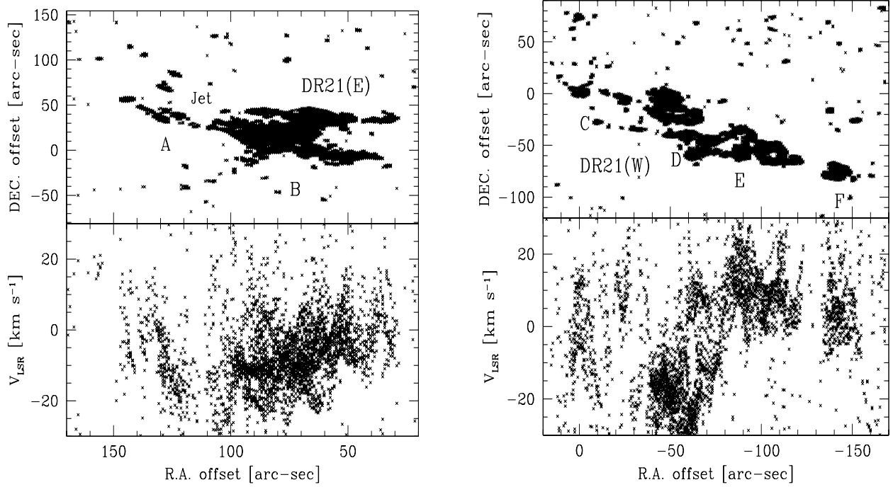
Fig. 6. Diagrams of detected \text{H}_2 v=1-0 S(1) line emission in all velocity channels (top) and the velocity-position diagrams (bottom) for DR 21 (E) (left) and DR 21 (W) (right). Offset values are referred to the position (0,0) of the driving source ( \text{HCO}^+ peak; Garden & Carlstrom 1992).
