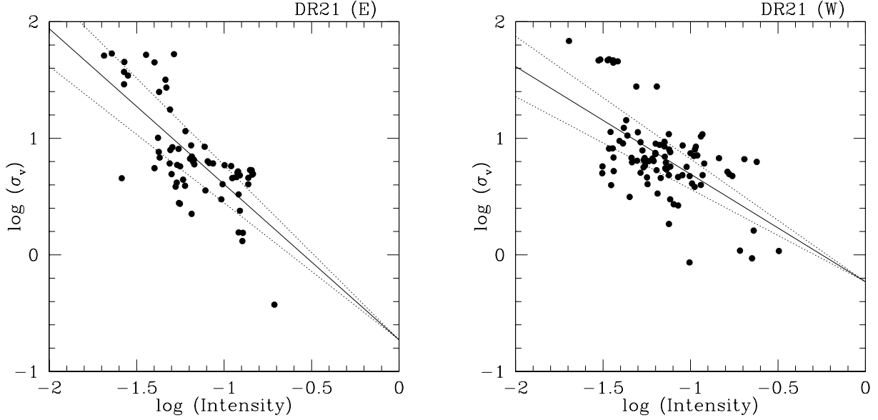
Fig. 10. The clump velocity dispersion \sigma_v vs. intensity I shows a power-law \sigma_v \propto I^c , where a large \sigma_v corresponds to fainter sources. DR 21 (E) is on the left and DR 21 (W) is on the right. The linear fit for each lobe is shown as a continuous line and the 1\sigma variations are shown as dotted lines. Slope values are c = -1.33 \pm 0.15 for DR 21 (E) and c = -0.92 \pm 0.15 for DR 21 (W).
