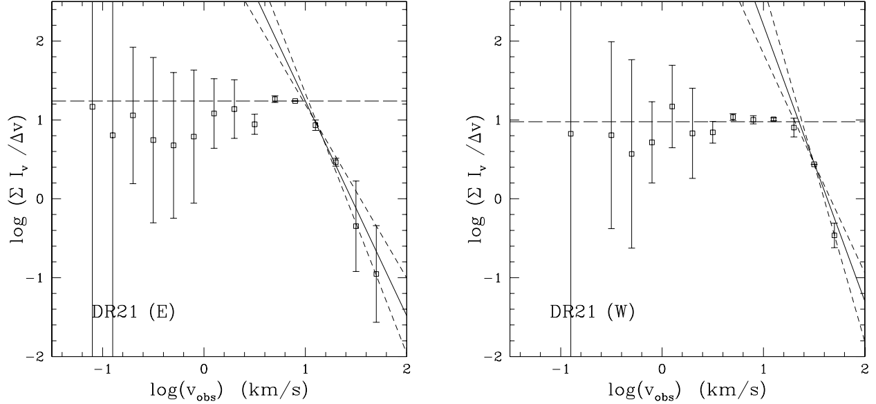
Fig. 5. Flux-velocity relation of H 2 S(1) v=1-0 S(1) emission in DR 21 (E) (left) and DR 21 (W) (right). The long-dashed line shows the flat low velocity behavior up to a break velocity, whereas the solid line indicates a power-law decrease. The short-dashed lines show the range of possible values of the power-law index, 2.7 \pm 0.55 for DR 21 (E) and 3.5 \pm 0.9 for DR 21 (W), and of \log(v_{break}) ( 1.00 \pm 0.03 and 1.35 \pm 0.03 , respectively).
