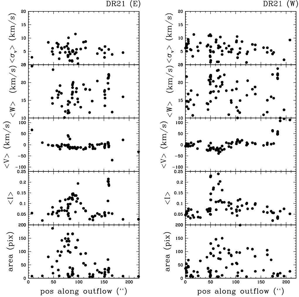
Fig. 8. Clump area and clump velocity moments along the outflow for DR 21. Each point on the graphs represents an identified clump along the outflow. From bottom to top the graphs present the area, intensity, centroid velocity, line width \langle W \rangle , velocity dispersion \sigma_v for each clump of DR 21 (E) (left) and DR 21 (W) (right).
