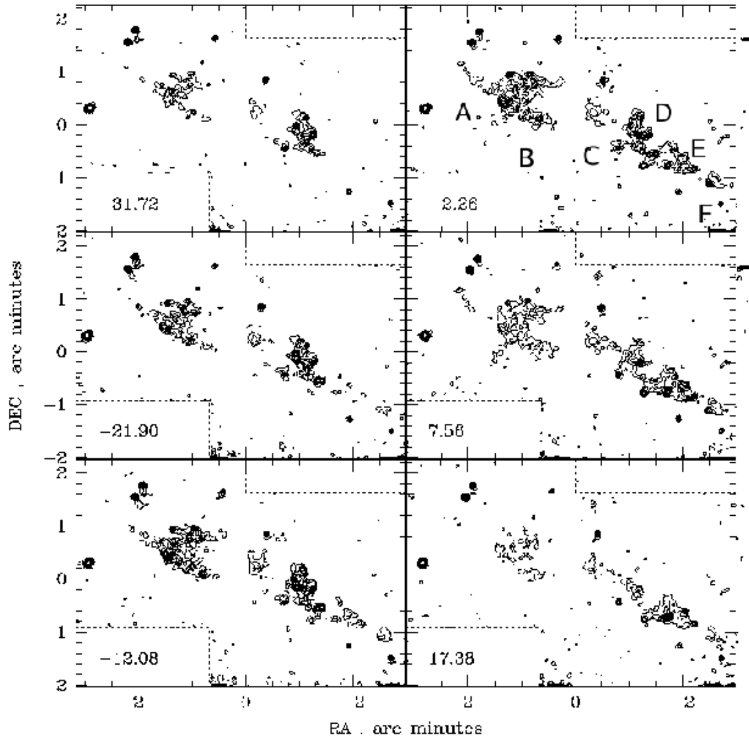
Fig. 1. Velocity channel maps of the \text{H}_2 v=1-0 S(1) line emission in DR 21, showing the radial velocity structure of the two regions DR 21 (E) and DR 21 (W). The velocity varies from -31.72 \text{ km s}^{-1} in channel 10 (top left) to +17.38 \text{ km s}^{-1} in channel 15 (bottom right), and the channel width is 9.8 \text{ km s}^{-1} . The minimum contour level is 0.12 \text{ counts s}^{-1} and the incremental values are 0.12 \text{ counts s}^{-1} . Regions with no observed data are marked by a dotted rectangle. The (0,0) position corresponds to that of the \text{HCO}^+ peak at RA(J2000.0) 203900.7, Dec(J2000.0) 421923.9 (Garden & Carlstrom 1992). Offsets are referred to this position.
