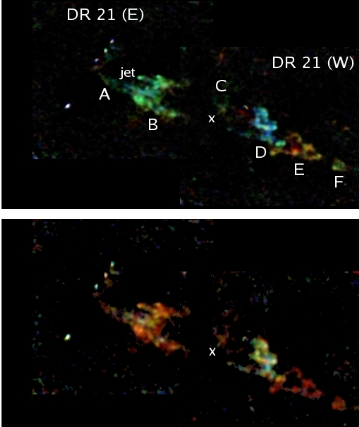
Fig. 2. Color composite of the Doppler-shifted H 2 v=1-0 S(1) 2.12 \mu\text{m} line emission in the outflow DR 21. Top: Image color corresponding to LSR velocities: blue -31.72 to -21.90 \text{km s}^{-1} , green -12.08 to -2.6 \text{km s}^{-1} , and red +7.56 to +17.38 \text{km s}^{-1} . Bottom: Image color corresponding to LSR velocities: blue -51.36 to -41.54 \text{km s}^{-1} , green -31.72 to -21.90 \text{km s}^{-1} , and red -12.08 to -2.6 \text{km s}^{-1} . The driving source adopted position is marked by X . Labels A to F are defined in the text. The region shown is about 7.0' \times 4.6' ( 5.1 pc \times 3.4 pc at distance D=2.5 kpc). The outflow extends on the sky \approx 6.5' which corresponds to a projected distance of 4.7 pc. North is at the top and east is to the left.
