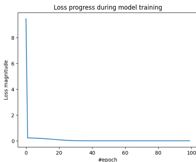
Figure 6. Loss Function
