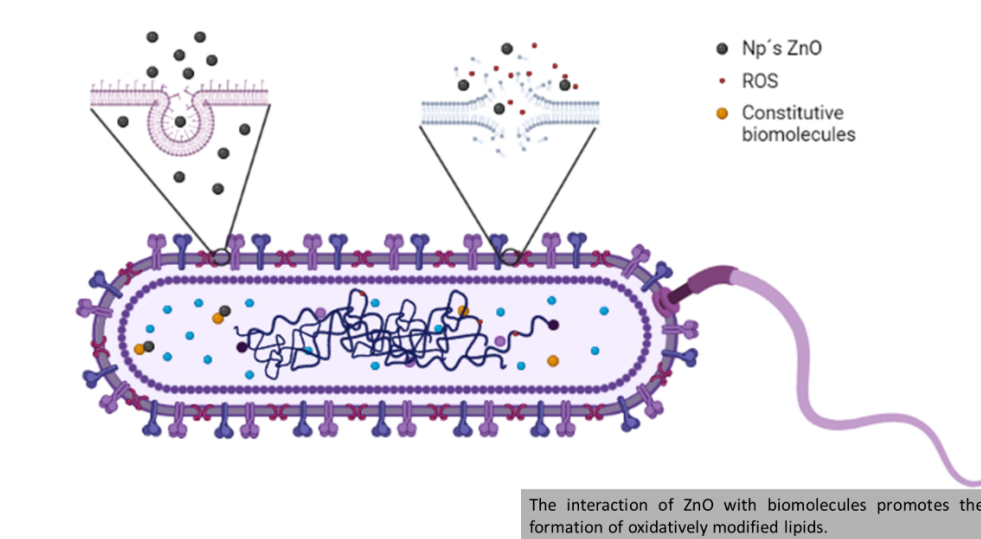
Figure 1. Scheme of proposed pathways for bacterial inhibition by ZnO nanoparticles.
