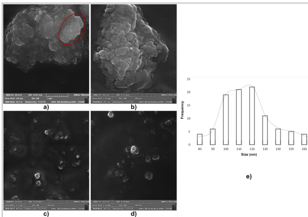
Figure 2. Micrographs of zinc oxide nanoparticles and particle size distribution; a) marks the area of the micrograph b), c) and d) random areas to measure individual particle size.
