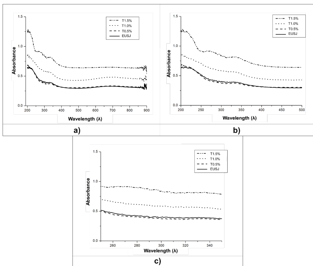
Figure 4. UV-vis spectrum of treatments and control (T0.05 %, T1.0 %, T1.5 %, EUSJ).
