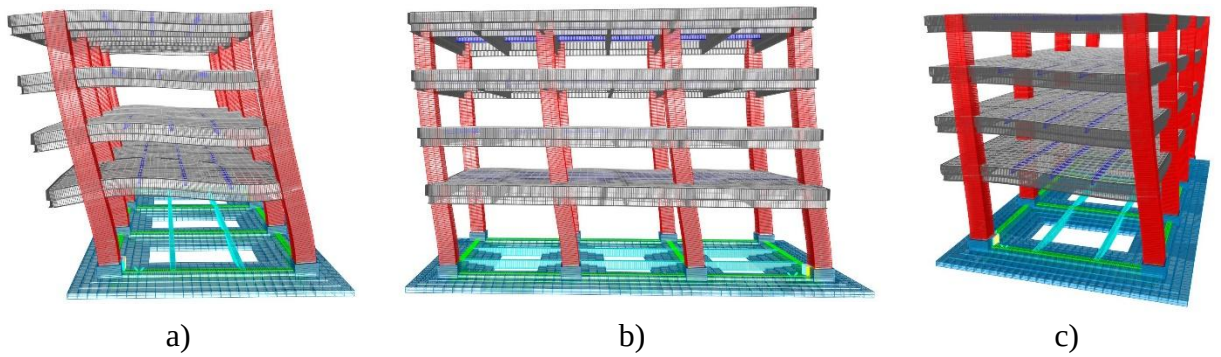
Figure 40. Vibration modes in SRTC; a) M1; b) M2; c) M3.
