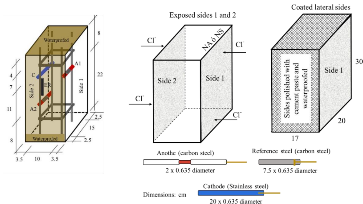
Figure 2. Scheme of the reinforced concrete specimens and embedded galvanic sensors.
