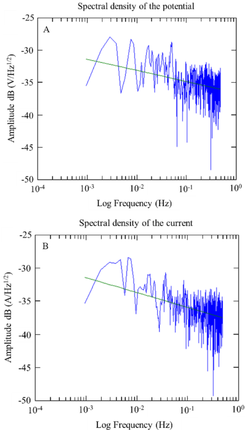
Figure 17. Spectral densities of potentials and currents over time were obtained from the A1 sensor, specifically at w/c 0.6 after 10 months of exposure.
