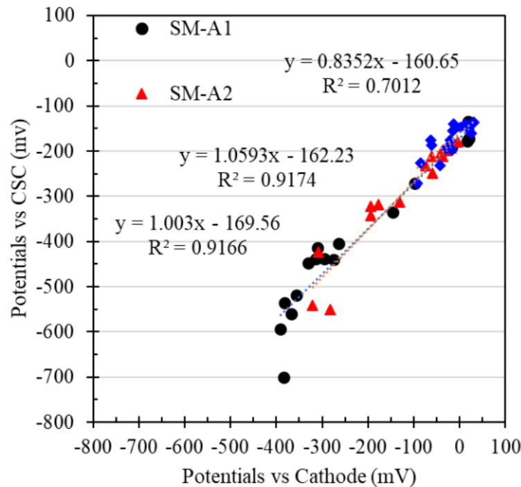
Figure 11. Comparison between the corrosion potentials vs. the cathode and the CSC electrode of the anodes of the test pieces with an a/c ratio of 0.4.
