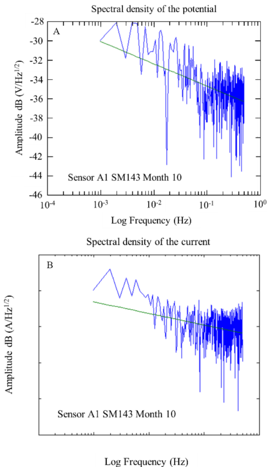
Figure 18. Spectral densities of potentials and currents over time were obtained from the A1 sensor, specifically at w/c 0.4 after 10 months of exposure.
