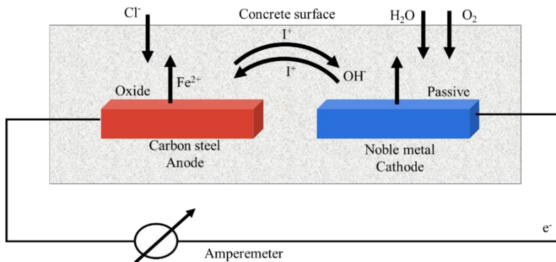
Figure 1. Corrosion Macrocell Scheme
