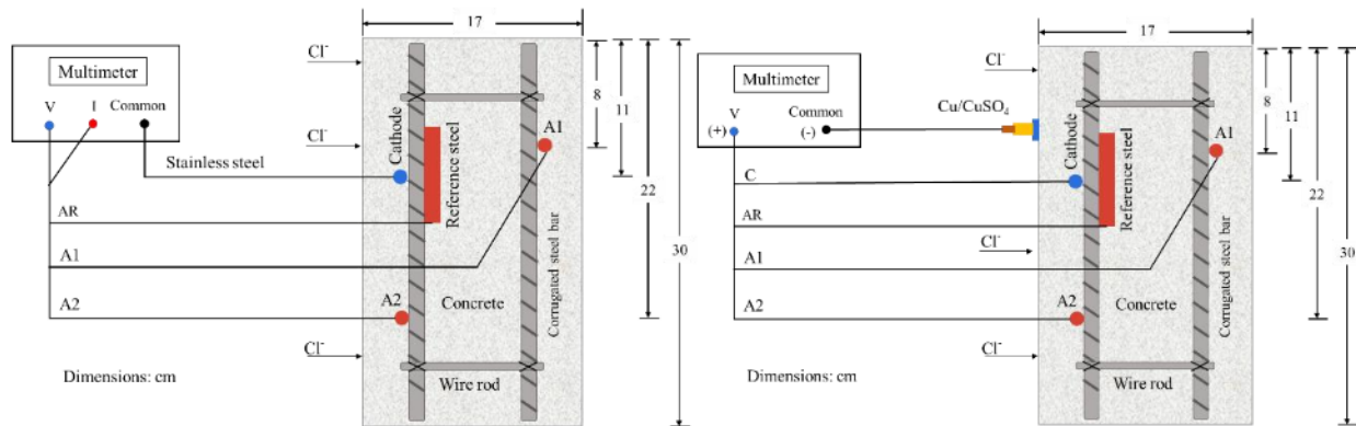
Figures 6a and 6b. Diagrams for monitoring Macrocell Voltages and Currents and Corrosion Potentials.
