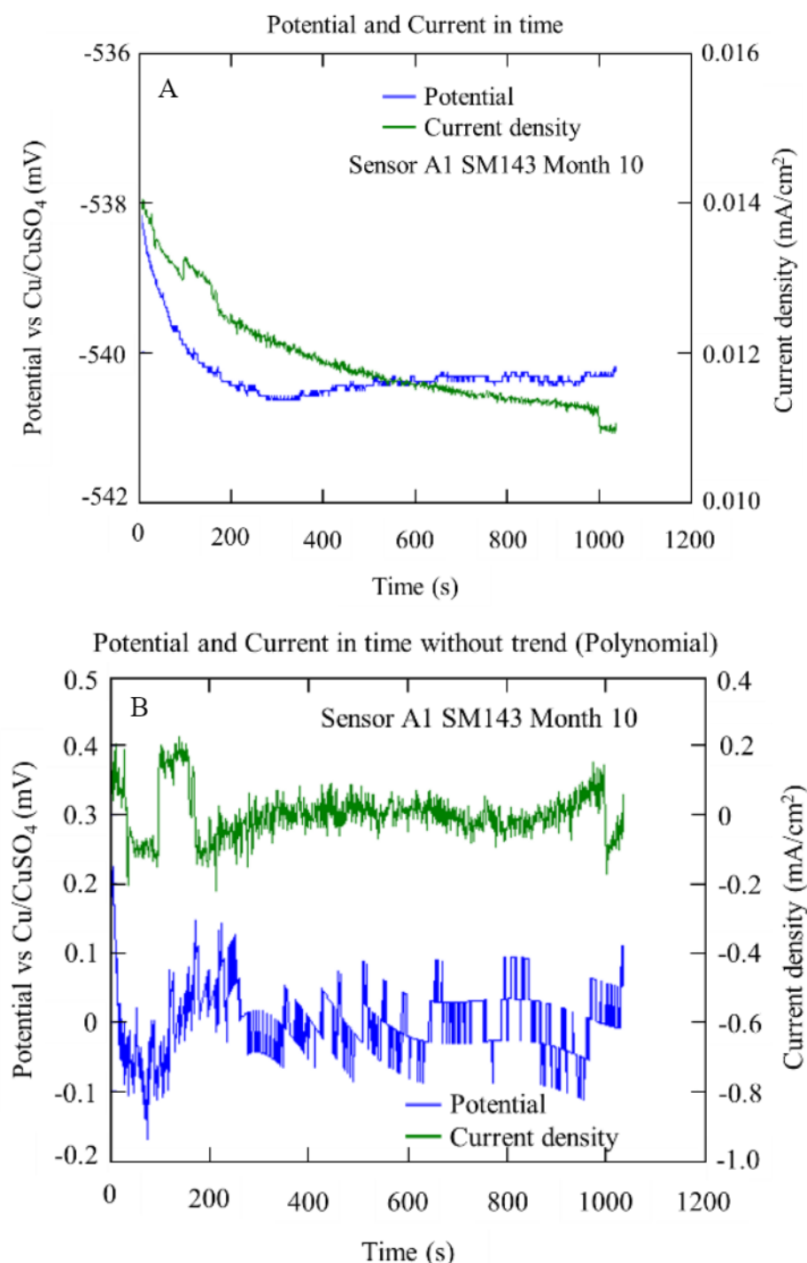
Figure 16. Potential and current series over time obtained from sensor A1 specifically with a/c 0.4, after 10 months in SM: with bias (A) and without bias (B)
