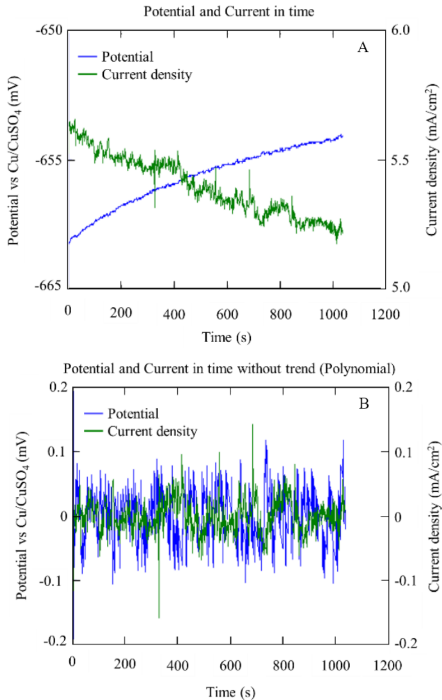
Figure 15. Series of potential and current over time obtained from anode A1 specifically with w/c 0.6, after 10 months in SM: with bias (A) and without bias (B).
