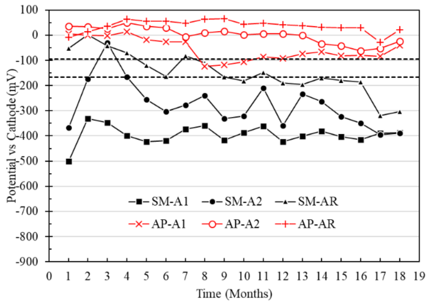
Figure 8. Potential vs. cathode specimens with a w/c ratio of 0.6 exposed in drinking water (AP) and 5% NaCl solution (SM).
