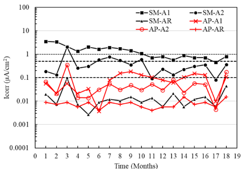
Figure 13. Macrocell current density of the specimens with w/c = 0.6 exposed to tap water (AP) and 5% NaCl solution (SM).
