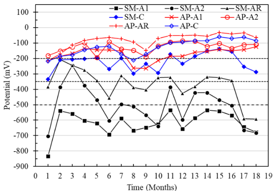
Figure 10. Potential vs. Cu/CuSO 4 from specimens with a w/c ratio of 0.6 exposed to drinking water (AP) and 5% NaCl solution (SM).
