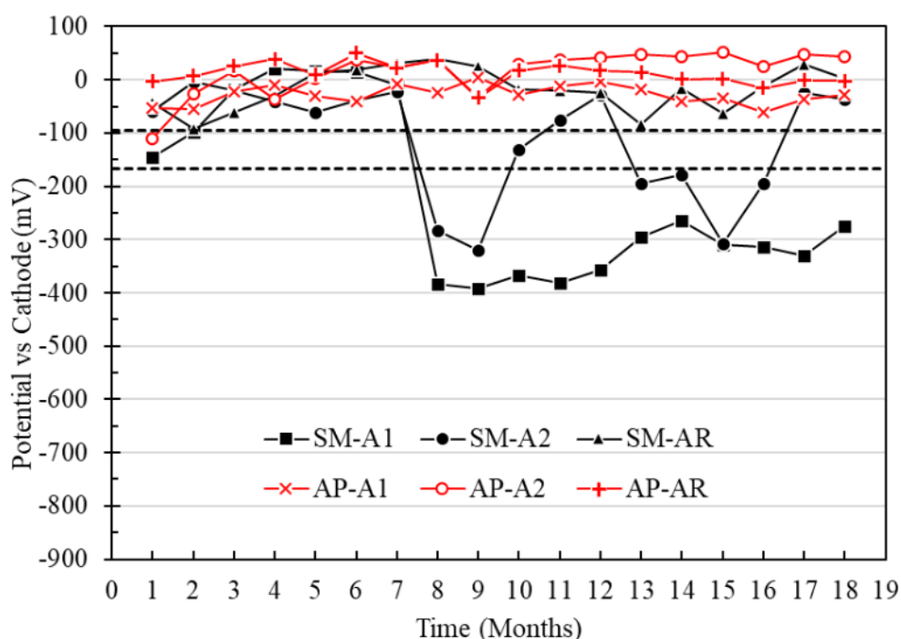
Figure 7. Potential vs. cathode of specimens with a w/c ratio of 0.4 exposed in tap water (AP) and 5% NaCl solution (SM).
