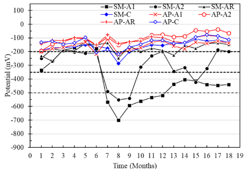
Figure 9. Potential vs. Cu/CuSO 4 from specimens with a w/c ratio of 0.4 exposed to drinking water (AP) and 5% NaCl solution (SM).
