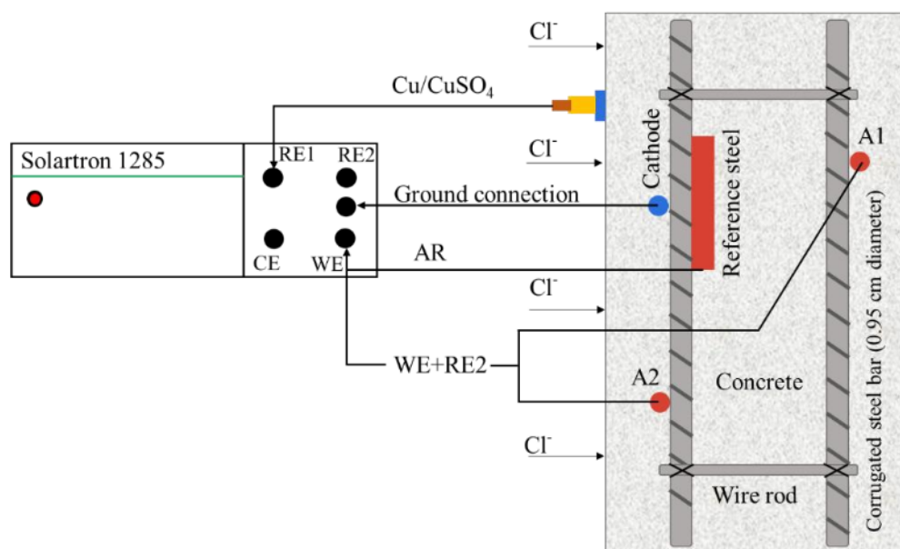
Figure 5. Diagram for monitoring Potential and Current in time
