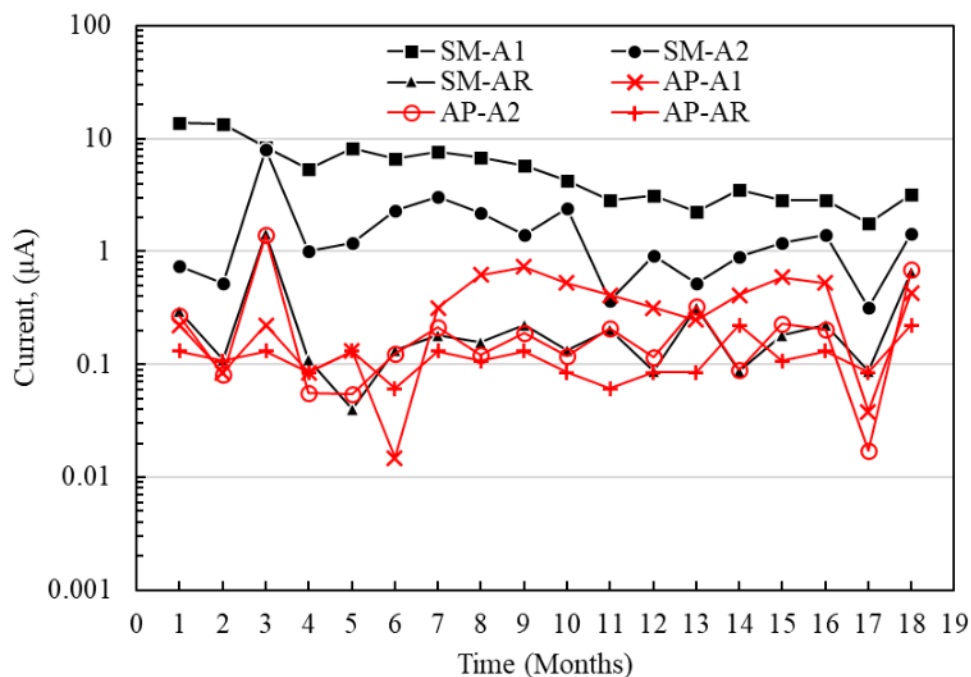
Figure 14. Macrocell current intensity of the specimens with a/c = 0.4 and 0.6 exposed to top water (AP) and 5% NaCl solution (SM).
