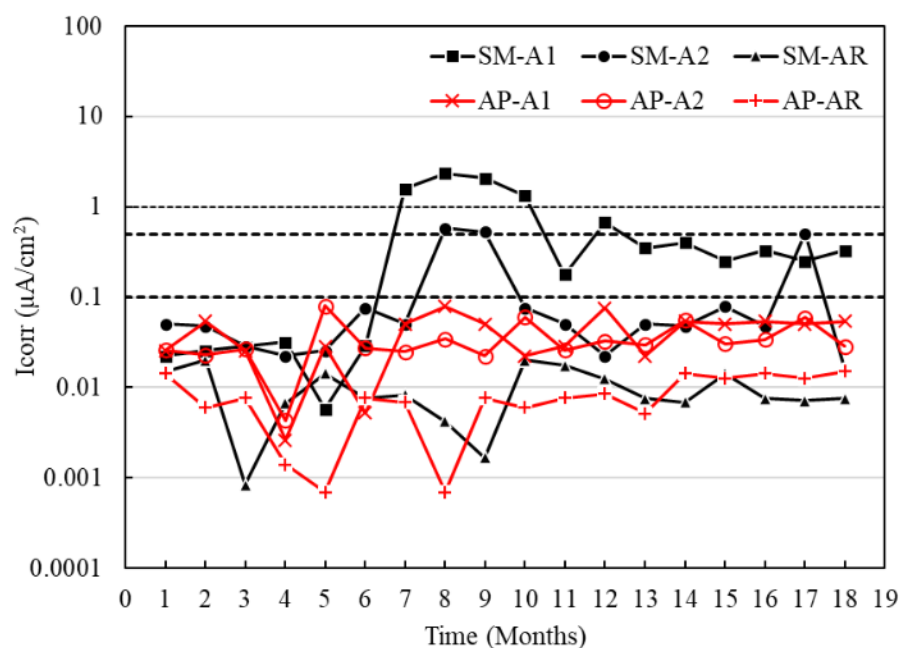
Figure 12. Macrocell current density of the specimens with w/c = 0.4 exposed to tap water (AP) and 5% NaCl solution (SM).
