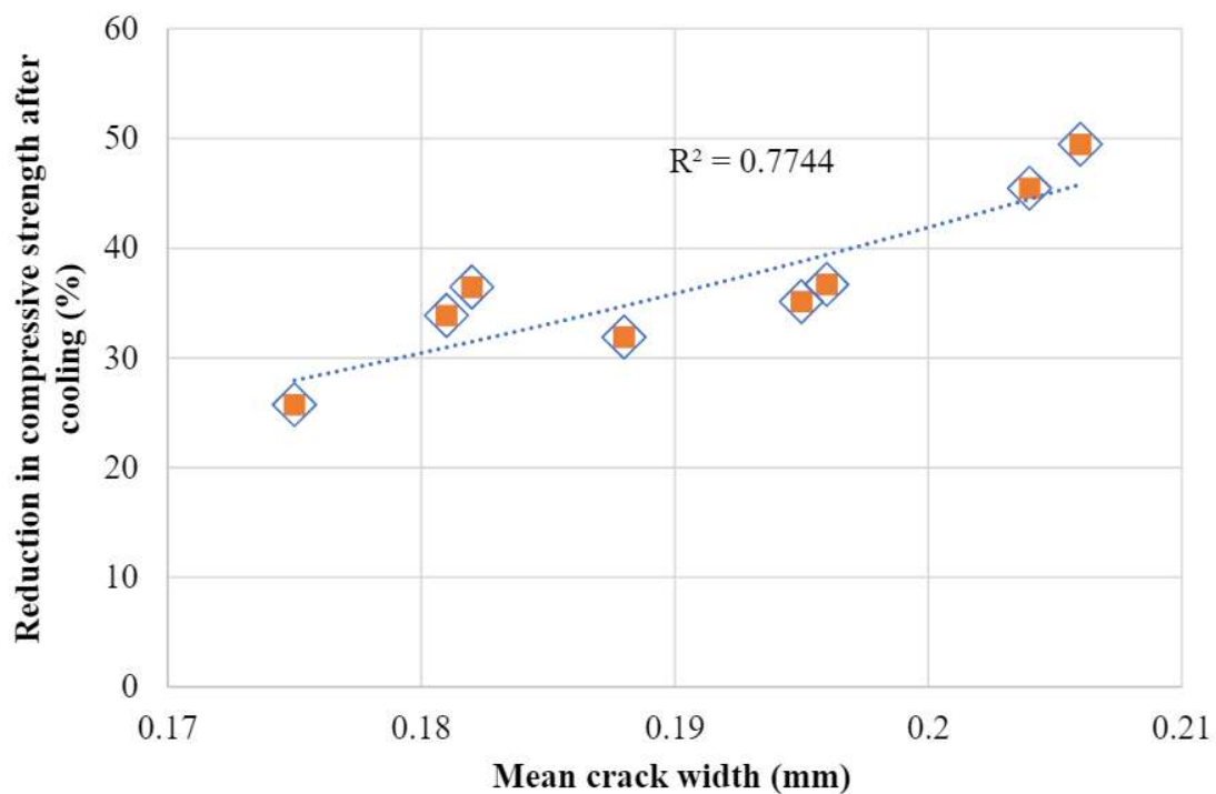
Figure 6. Relation between reduction in compressive strength and mean crack width after cooling.
