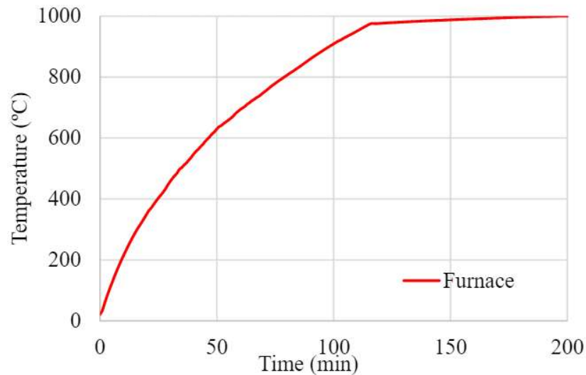
Figure 1. Heating procedure.
