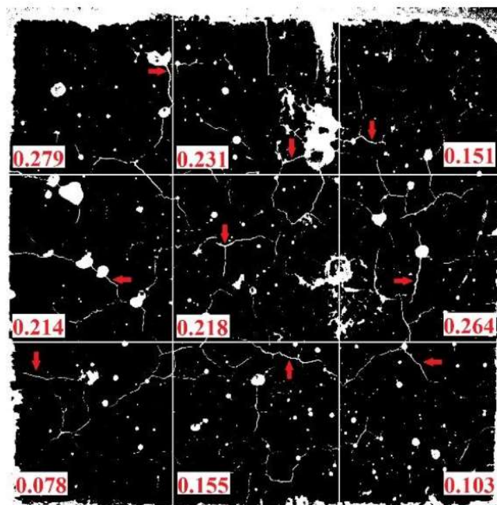
Figure 3. Crack width measurements on a C00X specimen (surface just after cooling).
