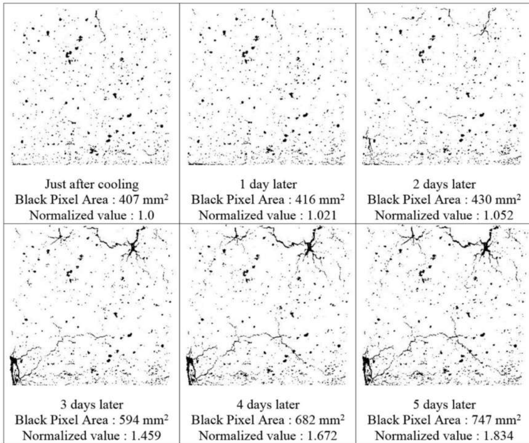
Figure 4. Crack growth monitoring on black and white images captured from COPZ specimen during air re-curing.
