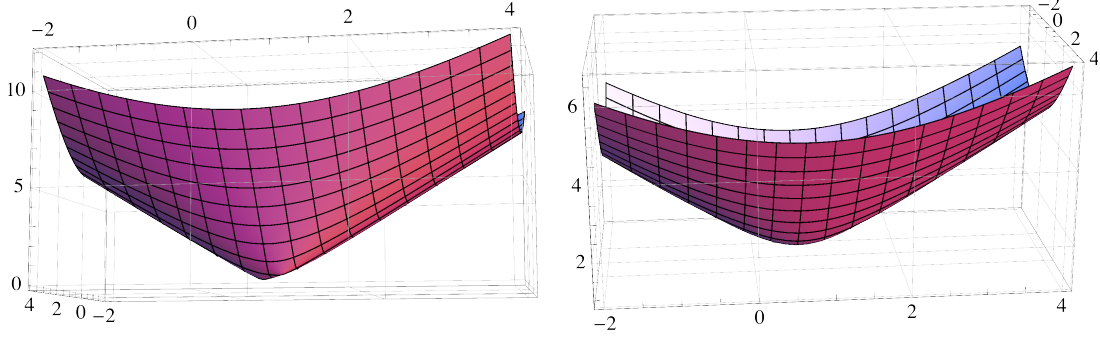
Fig. 2. Surface representation with (x, y, z) = (\text{Red}, \text{Zero}, \text{Blue}) and with (x, y, z) = (\text{Red}, \text{Green}, \text{Zero})
