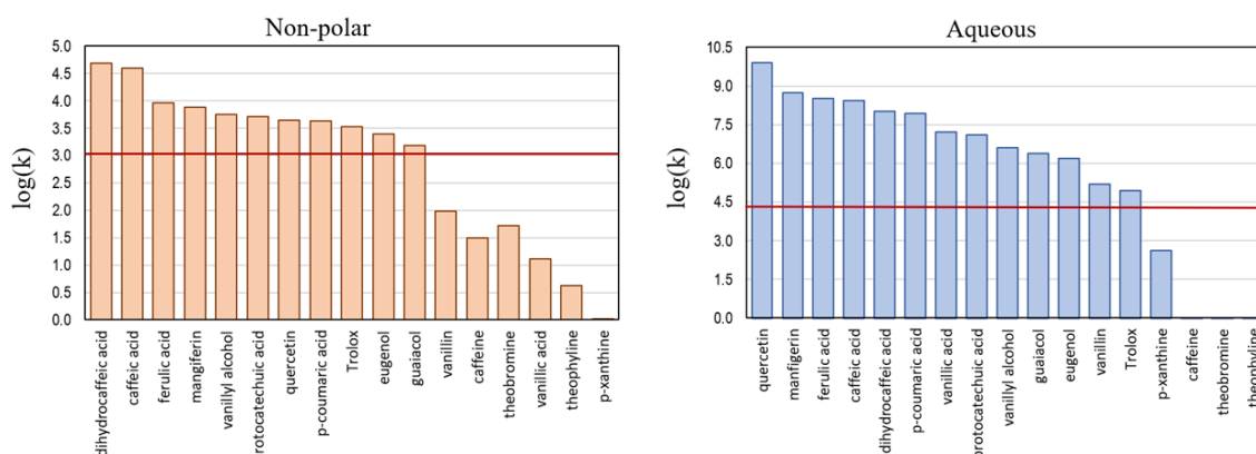
Fig. 3. \log(k) for the reactions between coffee components (and Trolox as reference) with \text{HOO}\cdot . The red line corresponds to the reaction of \text{HOO}\cdot with polyunsaturated fatty acids.
