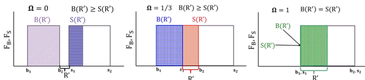
Fig. 2. Illustration of the first law of the DSBM. Each of the uniform distribution functions F_S and F_B satisfy the condition B(R') \geq S(R') , \forall R' > 0 . The values of B and S corresponds the shaded areas. b_1 (bonds) and s_1 (sites) denote the sizes of the smallest pore elements, whereas b_2 (bonds) and s_2 (sites) correspond to the sizes of the largest pore elements. Parameter \Omega represents the normalized area of overlap between F_B and F_S .
