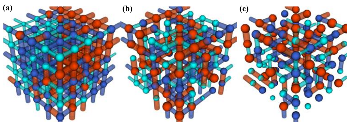
Fig. 11. Cubic networks with a high correlation are structured into regions measuring 5x5x5. (a) \bar{C} = 6 . (b) \bar{C} = 4 . (c) \bar{C} = 2 . Colors are utilized to create a contrast.
