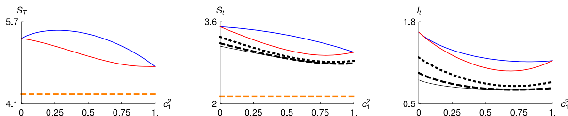
Fig. 6. Left: Plots of the Shannon pair entropic sum, S_T vs c_1^2 for the superposition function \Psi_{0111} , with attractive potential ( \lambda = 5 ), with (red curve) and without (blue curve) quantum interferences. The horizontal dashed line is the 2(1 + \ln \pi) uncertainty bound. Center: Plots of the reduced entropic sum S_t from the superposition function ( \lambda = 5 ) with (red curve) and without (blue curve) quantum interferences. The curves in black correspond to the superposition state with different values of \lambda (0-solid, 1-dashed, 2-dotted). The horizontal dashed line is the 1 + \ln \pi bound. Right: Plots of the information sum I_t vs. c_1^2 for the superposition function ( \lambda = 5 ) with (red curve) and without (blue curve) quantum interferences. Curves in black are as previously defined. The value of \omega is set at unity in all curves.
