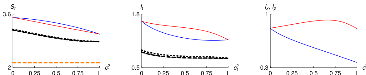
Fig. 7. Left: Plots of the reduced entropic sum, S_t , from the superposition function \Psi_{0111} , with repulsive potential ( \lambda = 0.7 ), with (red curve) and without (blue curve) quantum interferences. The curves in black correspond to the superposition state with different values of \lambda (0-solid, 0.25-dashed, 0.5-dotted). The horizontal dashed line is the 1 + \ln \pi bound. Center: Plots of the information sum I_t vs. c_1^2 for the superposition function ( \lambda = 0.7 ) with (red curve) and without (blue curve) quantum interferences. Curves in black are as previously defined. Right: Plots of the I_x (red curve) and I_p (blue curve) components with \lambda = 0.7 vs. c_1^2 . The value of \omega is set at unity in all curves.
