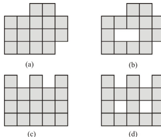
Figure 3. Shapes Used to Numerically Validate Theorems 1 and 2(a).
