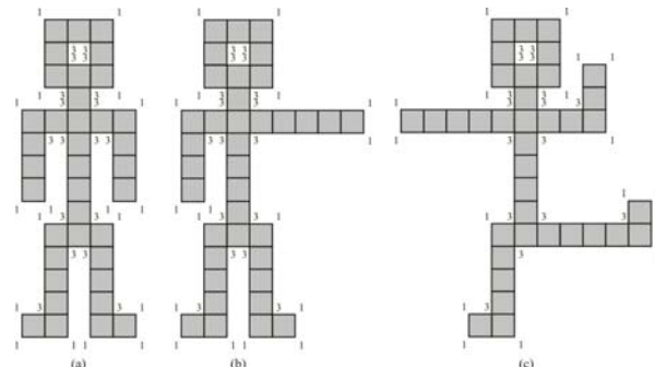
Figure 5. The Euler Number of a Shape Remains Unchanged if its Topology Does not Change.
