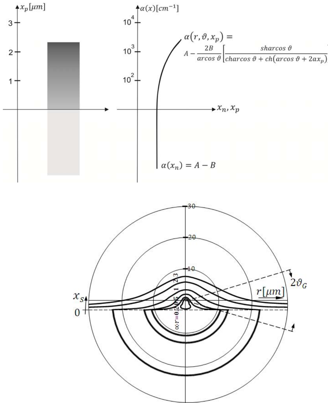
Figure 3. Radiation field around a point source. Full line: curves of constant intensity. Distance of the emitter from the interface, x_p = 3\mu\text{m} , r -length of radius vector between the excitation point (x_p, y_p, z_p) and the point of observation. \vartheta – angle between x direction and \vec{r} , \vartheta_G – limiting angle. Absorption function is due to Equation (11). The solid curves correspond to values \alpha \cdot r = 0.2; 0.5; 1; 2; 3
