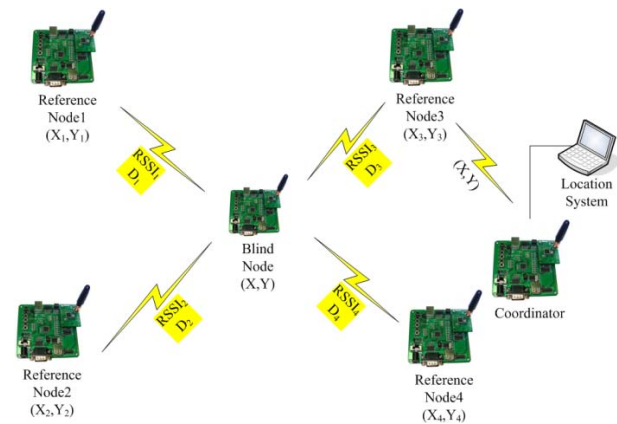
Figure 1. A scenario of the ZPS scheme for estimating the BN's location based on the RSSI information.
