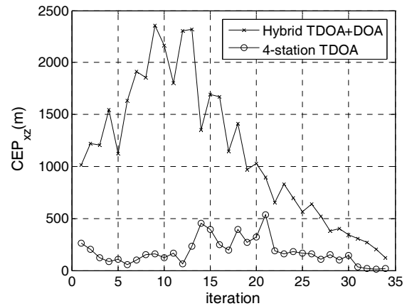
Figure 5. CEP_{xz} comparison.
