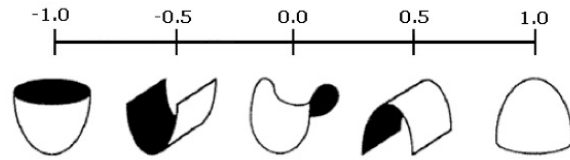
Figure 5. Representation of local forms in the Shape Index classification.
