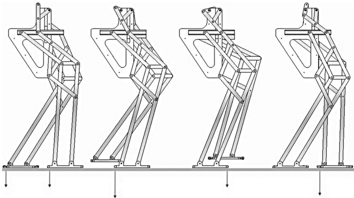
Figure 5. Mimbot with the new stabilization system. Phases: double support, start of the foot lifting, foot descent, contact with the ground.
