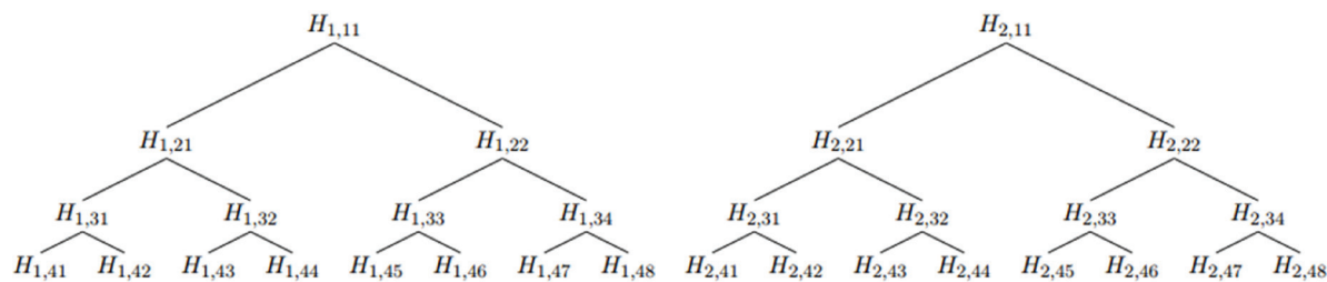
Figure 2. A Merkle tree chain
