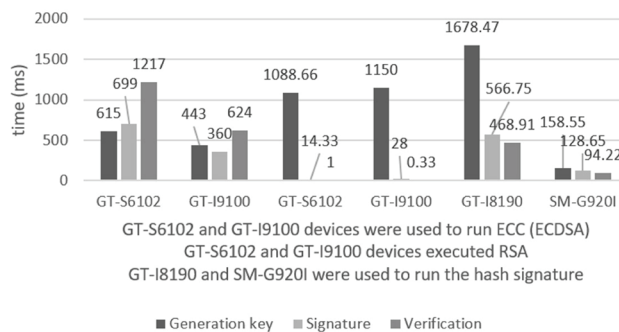
Figure 4. The hash signature system SHA-256 is compared to Tayoub et al. (2013). These results show that the hash signature system 256-bit, running in the SM-G9201 device is faster than ECC (ECDSA) 224-bit and RSA 1024-bit when comparing the time required for key generation, signature and verification
