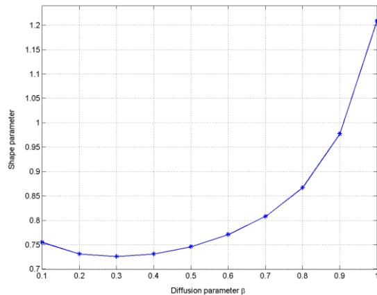
Figure 8. Variation of the shape parameter with respect \beta , fixed \epsilon = 0.5
