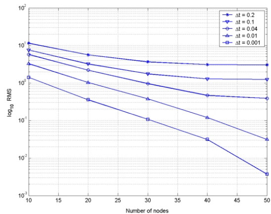
Figure 5. Convergence for fixed \beta=0.2 and \mu=1 with different time steps at time t_{max}=1 with implicit multiquadric
