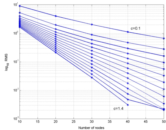
Figure 7. Variation of the shape parameter with \rho=0.1 , \mu=0.2 , at time t_{max}=1
