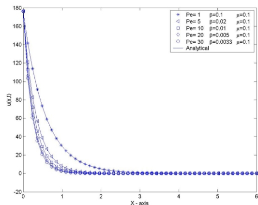
Figure 2. Analytical and numerical solution with different values of b , at time t_{\max}=1
