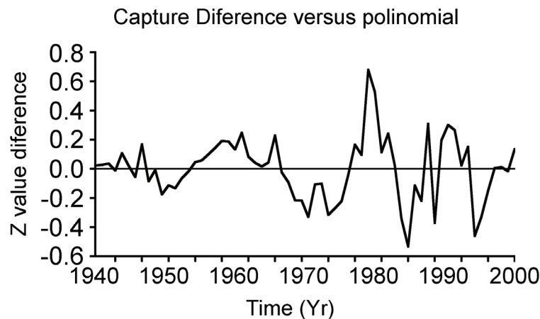
Figure 4. Z standardized values of the difference between the observed landings and the polynomial computed data (z-landings). Z is defined as (x' - \bar{x})/\sigma , where \bar{x} is the average, x_i the i -th landing difference data, and \sigma the standard deviation).
