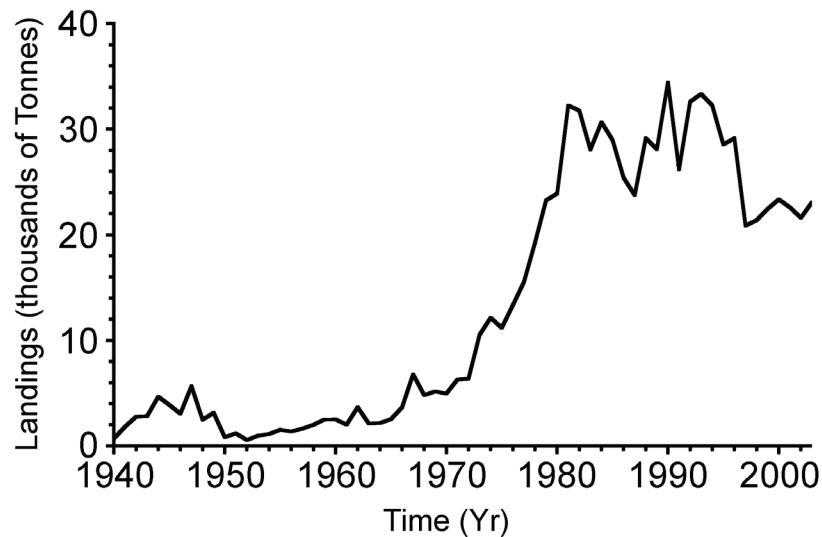
Figure 1. Time series (Yr) of sharpnose ( Rhizoprionodon terraenovae ) landings (thousands of tons) in the Gulf of Mexico between 1940 and 2003. There has been a strong increase in landings since the late 60s.
