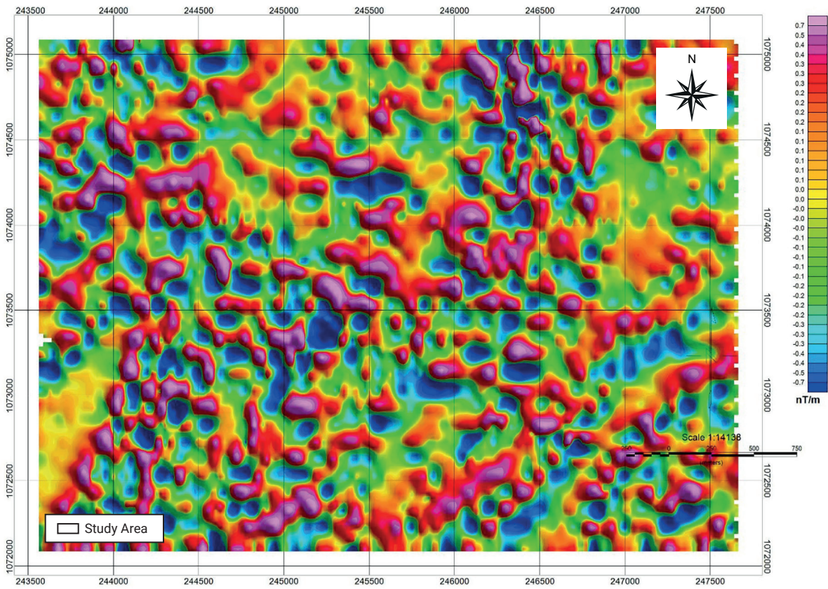
Figure 5. First Vertical Derivative map.
