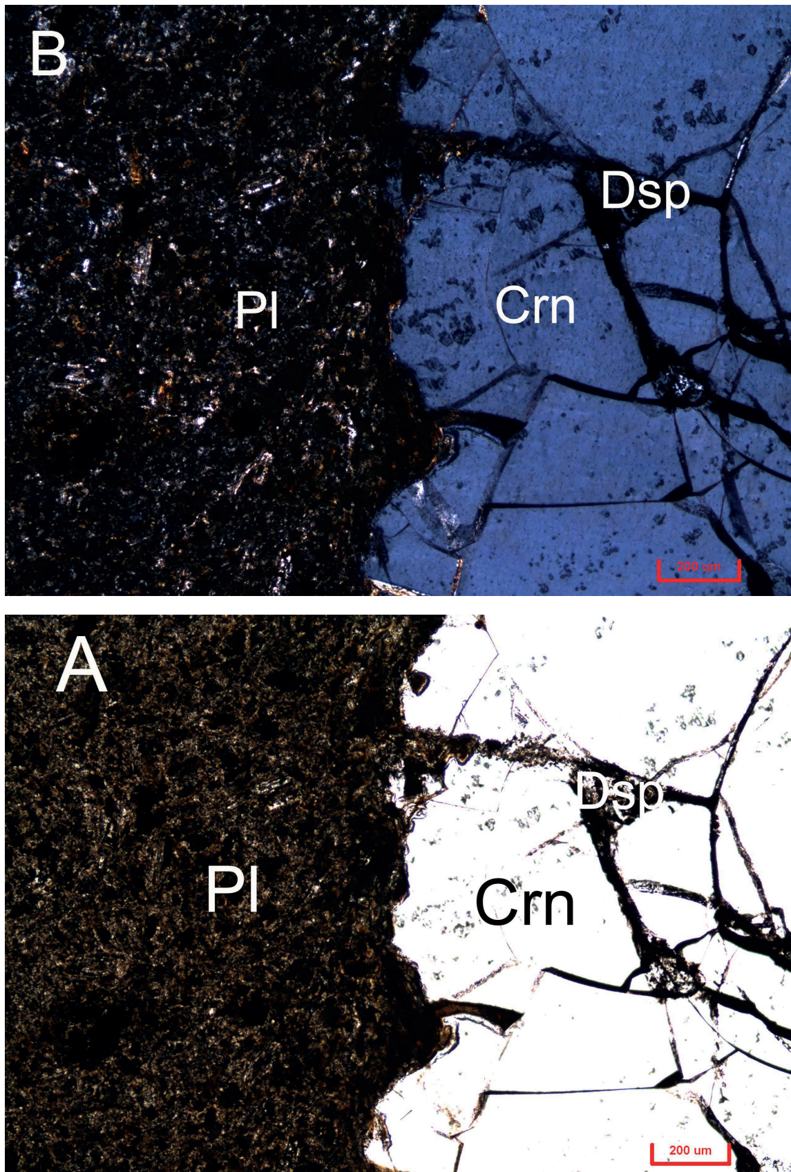
Figure 3. Photomicrographs showing the petrographic characteristics of the studied dacite and ruby xenocrysts, 5X; A = PPL; B = XPL. Plagioclase phenocrystals (PI), are observed with partially vitreous microlithic matrix and fractured anhedronal ruby phenocrysts (Crn) with incipient alteration to diaspore (Dsp).
