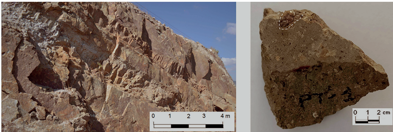
Figure 2. Photographs showing the outcropping dacitic lava host rock and a rock sample of centimeter scale ruby xenocrysts (Dotted half circle). The lava flow is pseudostratified, altered, and jointed.
