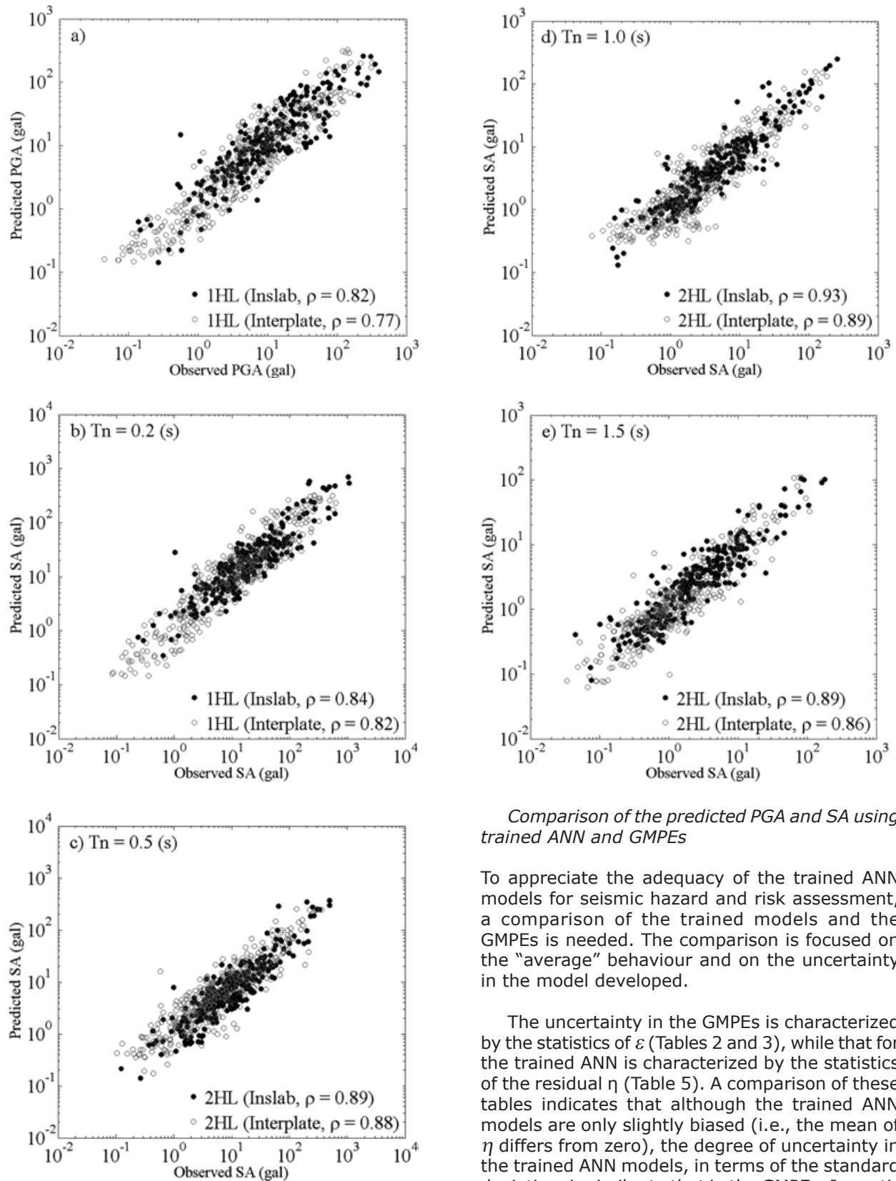
Figure 7. Comparison of predicted and observed PGA and SA H1 component values for inslab and interplate earthquakes ( \rho in the plots denotes correlation coefficient).
