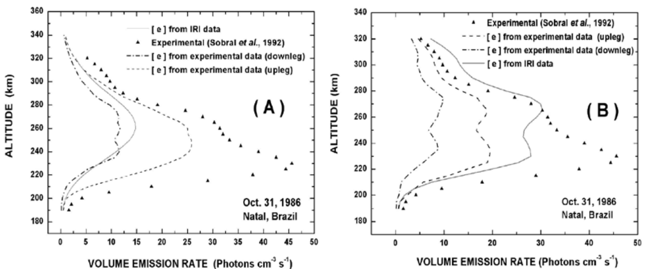
Fig. 3. Comparison between OI 630 nm red line volume emission rate profiles derived from the experiment carried out in October 31, 1986 (Sobral et al. , 1992) and calculated profiles. ( A ) The theoretical profiles with constant quantum yield f(^1D) \sim 1.2 (Link and Cogger, 1988) were evaluated from experimental data of electron density (upleg and downleg) and IRI electron density data. ( B ) The theoretical profiles with height-dependent profile for f(^1D) obtained from Sobral et al. (1992) were also evaluated from experimental data of electron density (upleg and downleg) and IRI electron density data.
