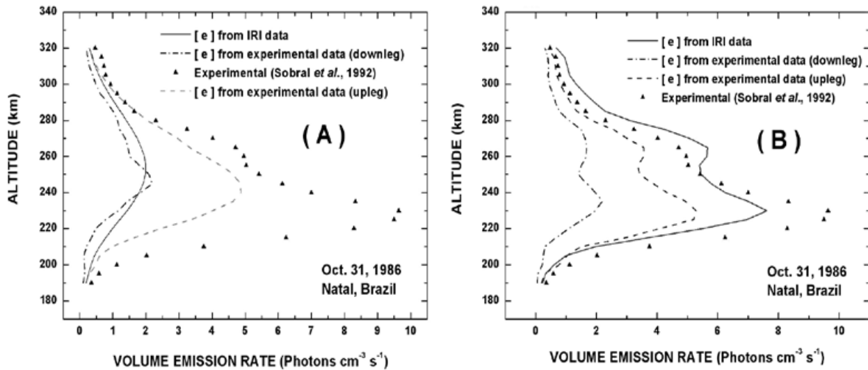
Fig. 2. Comparison between OI 557.7 nm green line volume emission rate profiles derived from the experiment carried out in October 31, 1986 (Sobral et al. , 1992) and calculated profiles. ( A ) The theoretical profiles with constant quantum yield f(^1S) = 5.0 \times 10^{-2} (Takahashi et al. , 1990) were evaluated from experimental data of electron density (upleg and downleg) and IRI electron density data. ( B ) The theoretical profiles with height-dependent profile for f(^1S) obtained from Sobral et al. (1992) were also evaluated from experimental data of electron density (upleg and downleg) and IRI electron density data.
