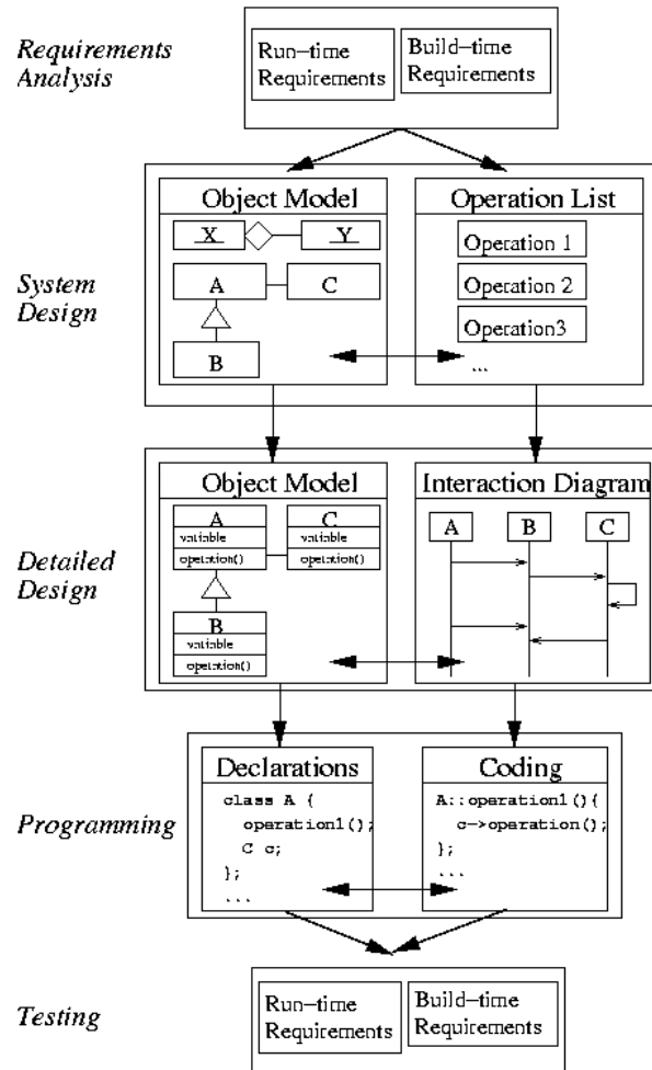
Fig. 4. Phases of the Practical Design Method
