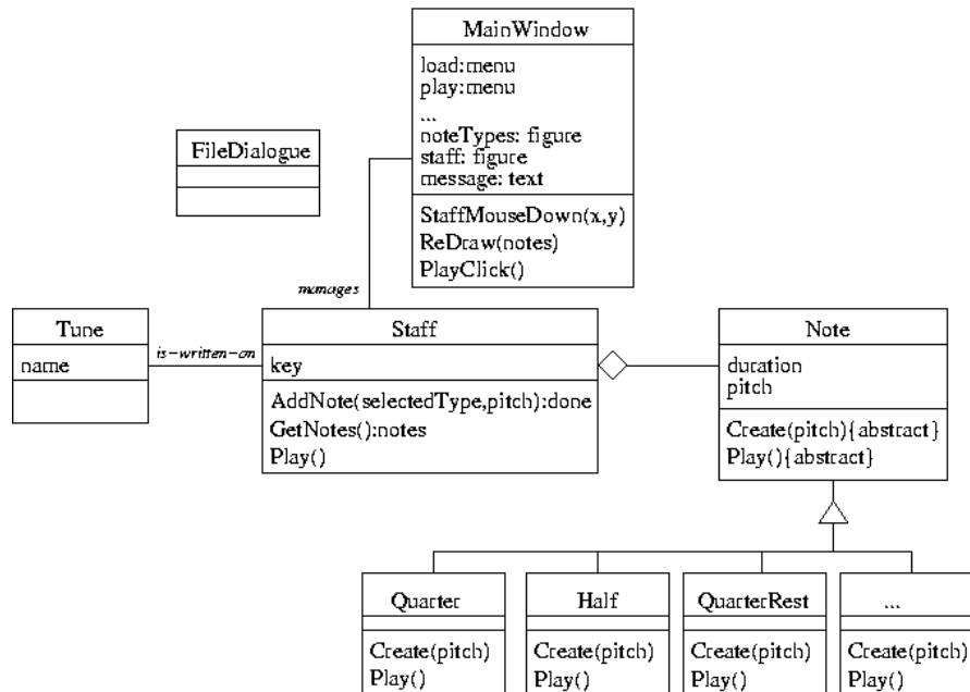
Fig. 14. Class diagram for a third version of the Elementary Composer
