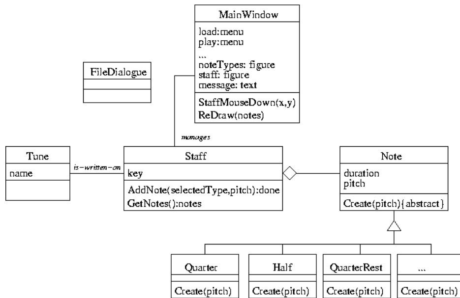
Fig. 12. Class diagram for a second version of the Elementary Composer
