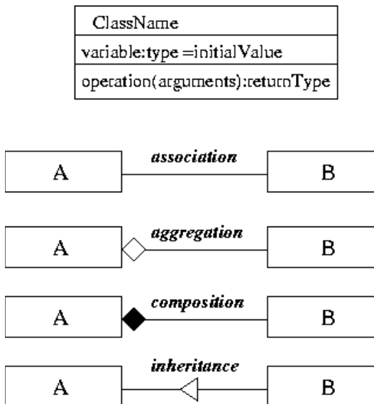
Fig. 2. Basic elements of a Class Diagram
