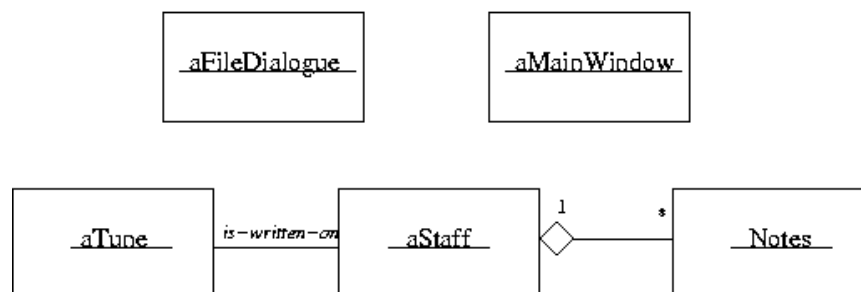
Fig. 7. Object diagram for the first version of the Elementary Composer example
