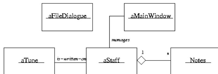
Fig. 11. Object diagram for a second version of the Elementary Composer
