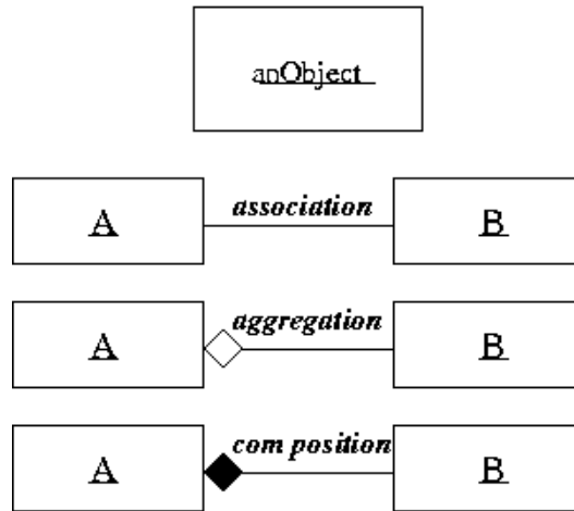
Fig. 1. Basic elements of an Object Diagram
