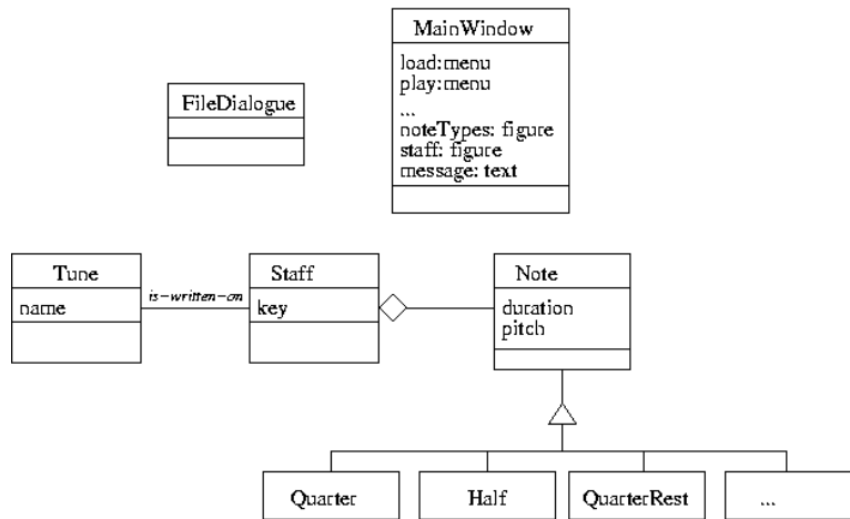
Fig. 8. Class diagram for the first version of the Elementary Composer example
