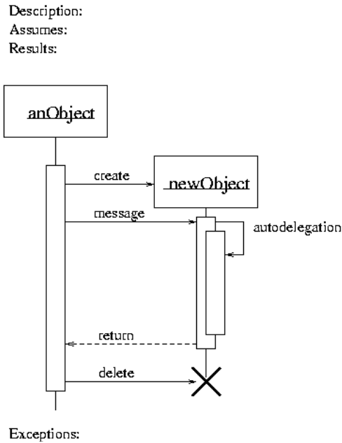
Fig. 3. Notation for an Interaction Diagram
