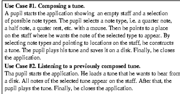
Fig. 5. Use cases as run-time requirements for the “Elementary Composer” example application
