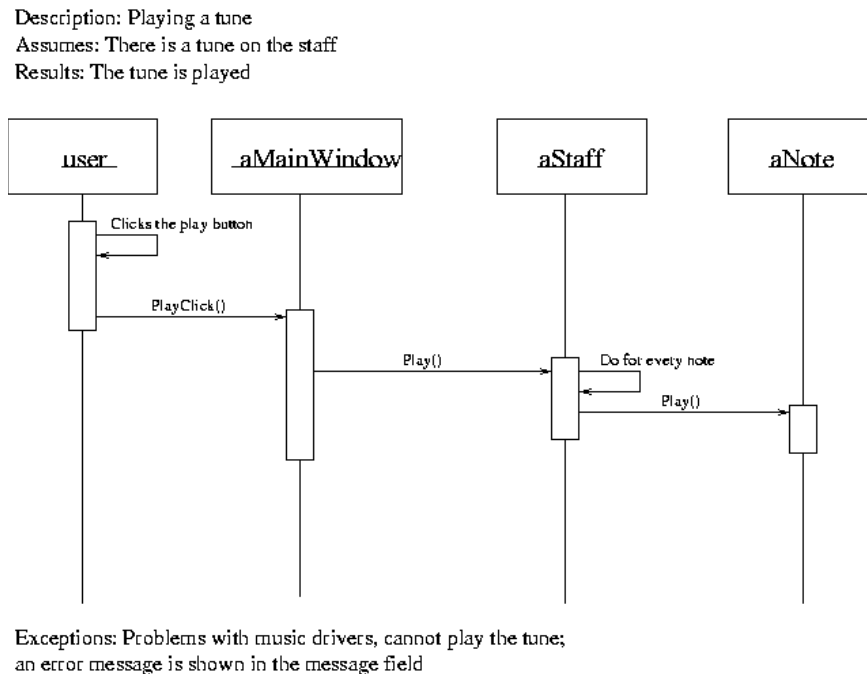
Fig. 13. Interaction diagram for “playing a tune” operation
