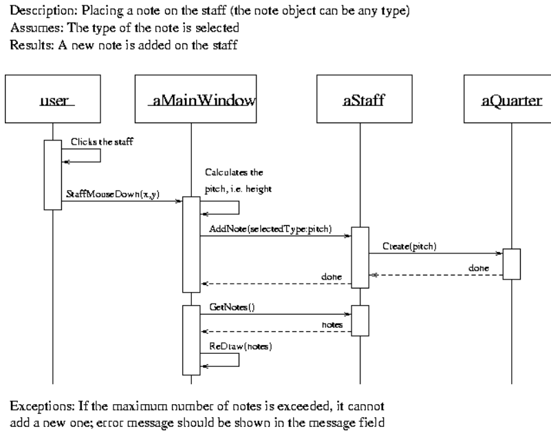
Fig. 10. Interaction diagram for “placing a note on the staff” operation
