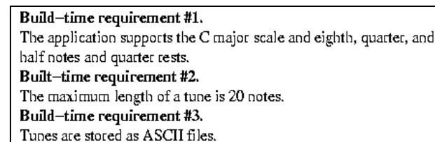
Fig. 6. Build-time requirements for the “Elementary Composer” example application
